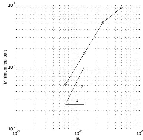
Fig. 5. Minimum real parts of eigenvalues of the Schur complement, for streamline-upwind discretization on a 64 \times 64 grid.
