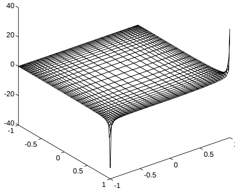
Fig. 4. Pressure solution for \nu = 1/10 .
