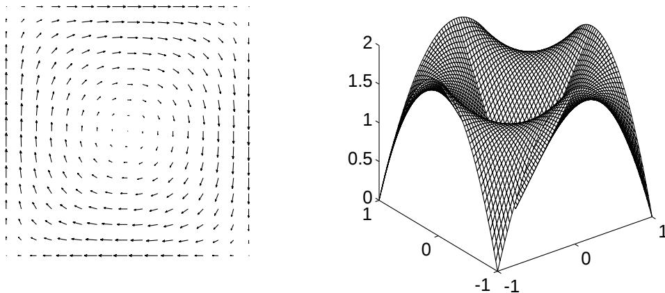
Fig. 1. Magnitude and direction of the convecting flow.
