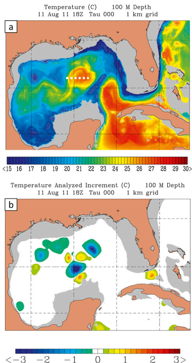
FIG. 6. (a) Ocean temperatures ( ^{\circ}\text{C} ) at 100-m depth from the 1800 UTC 11 Aug 2011 HYCOM analysis (including AXBT data). White dashed line highlights the AXBT deployment locations along 26^{\circ}\text{N} . (b) Increment ( ^{\circ}\text{C} ) in HYCOM ocean temperature at 100 m, which is the AXBT observation temperature minus the model background. The pattern suggests the AXBT data both strengthened the magnitude (along 26^{\circ}\text{N} ) and reduced the NE–SW extent of the WCR in the model.
