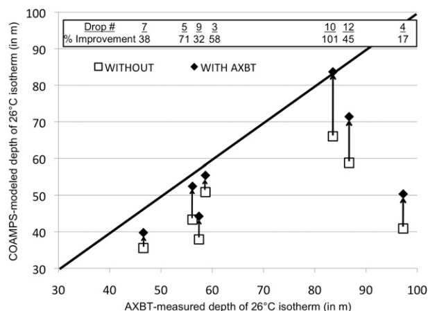
FIG. 12. Comparison of COAMPS-TC (modeled) vs AXBT (observed) depths of 26^{\circ}\text{C} isotherm for the COAMPS-TC 1200 UTC 27 Aug 2011 analyses without (clear squares) and with (black diamonds) AXBT data. The black diagonal line marks the location where the model value equals the observed value. Black arrows indicate the change in the model following initialization with the AXBT data. Percent improvement for each drop is noted in the text box at the top.
