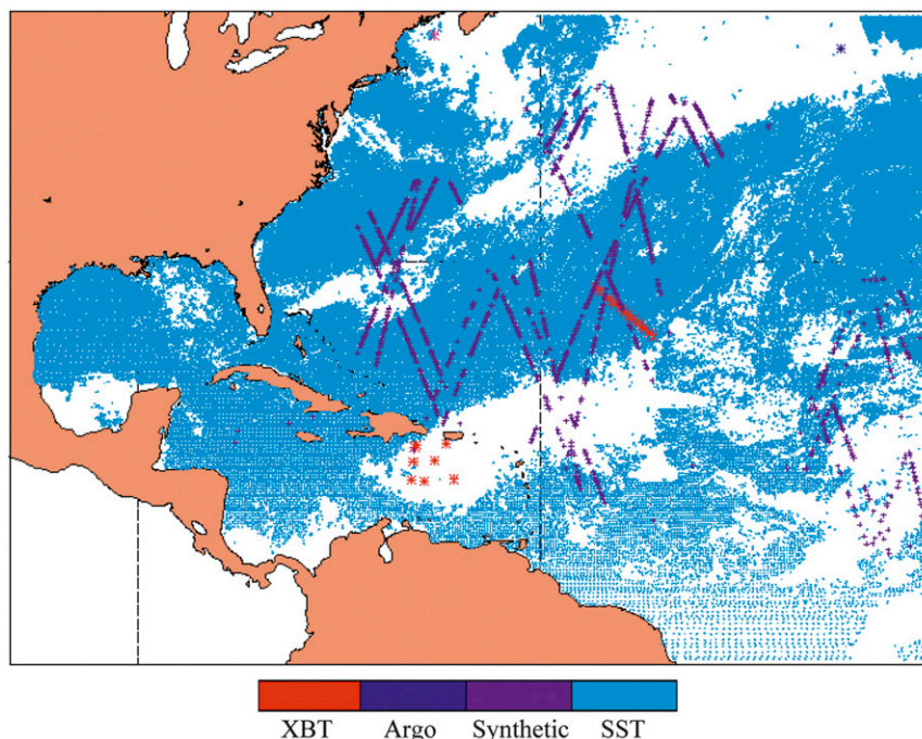
FIG. 2. Locations of ocean temperature observations (colors indicate observation source) assimilated by the NCODA system at 1200 UTC 3 Aug 2011. Grid spacing is 6 km. Eight of the 11 AXBTs deployed beneath TS Emily as part of the 2011 AXBT Demonstration Project filled the data-void region southeast of the Dominican Republic in near-real time.
