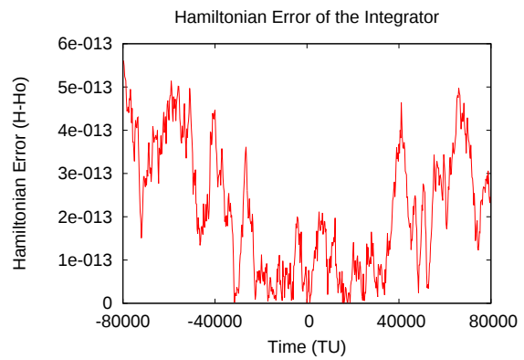
Figure A.8: Hamiltonian Error, TC1-6
