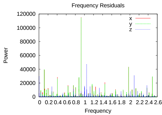
Figure B.5: Frequency Residuals, TC1-3
