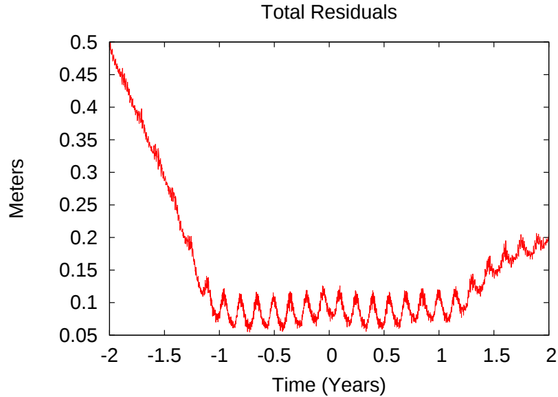
Figure 4.5: TC1-1 Position Residuals
