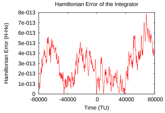
Figure A.6: Hamiltonian Error, TC1-4
