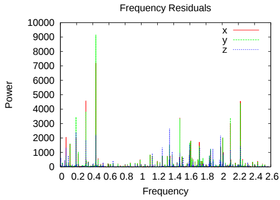
Figure B.1: Frequency Residuals, TC0-1
