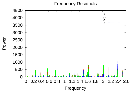
Figure B.3: Frequency Residuals, TC1-1
