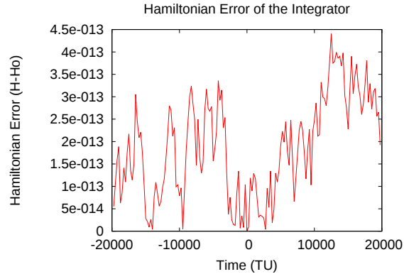
Figure A.2: Hamiltonian Error, TC0-2
