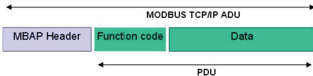
Figure 2.4: MODBUS/TCP ADU [Mod06]
