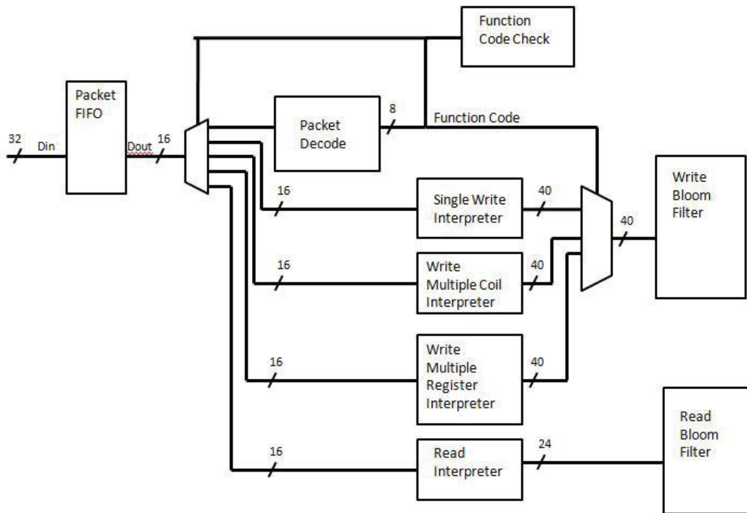
Figure 3.3: Simplified Block Diagram of the MODBUS Inspection Core
