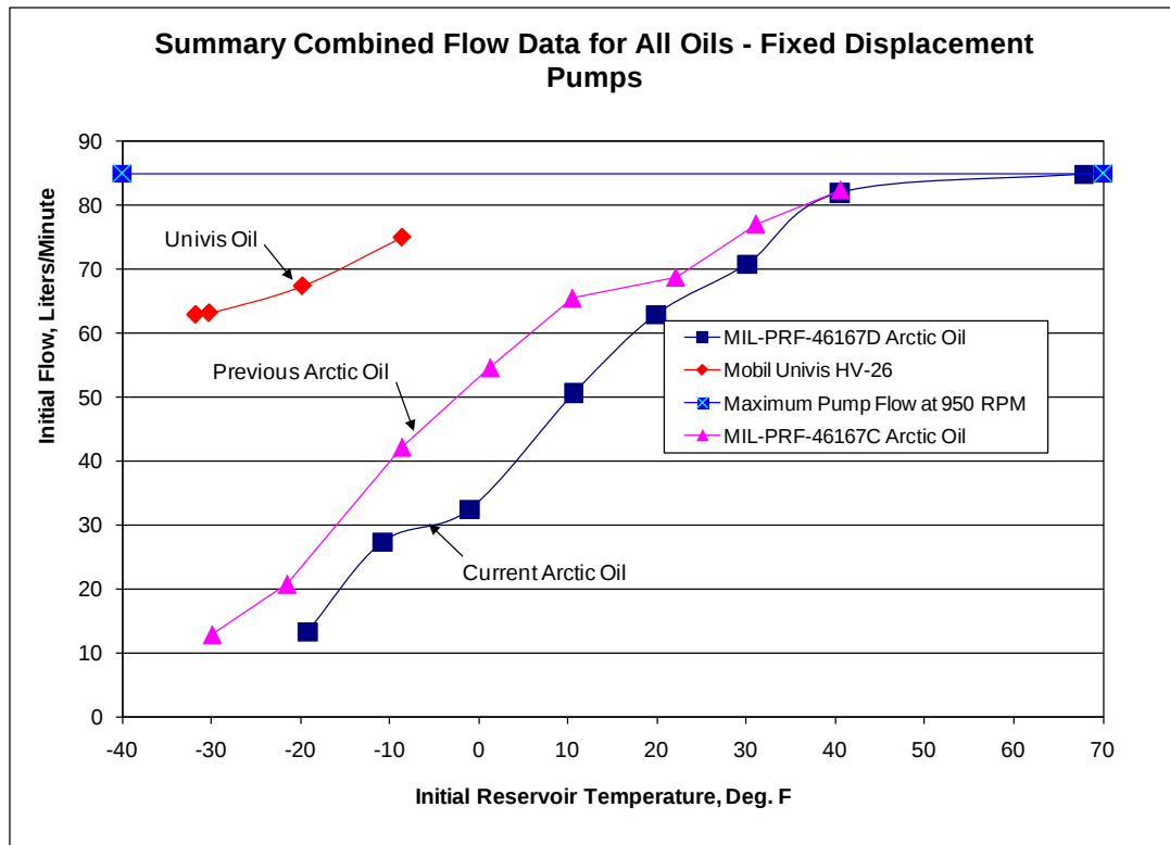
Figure 12. Summary Combined Flow Data for All Oils – Fixed Displacement Pumps
