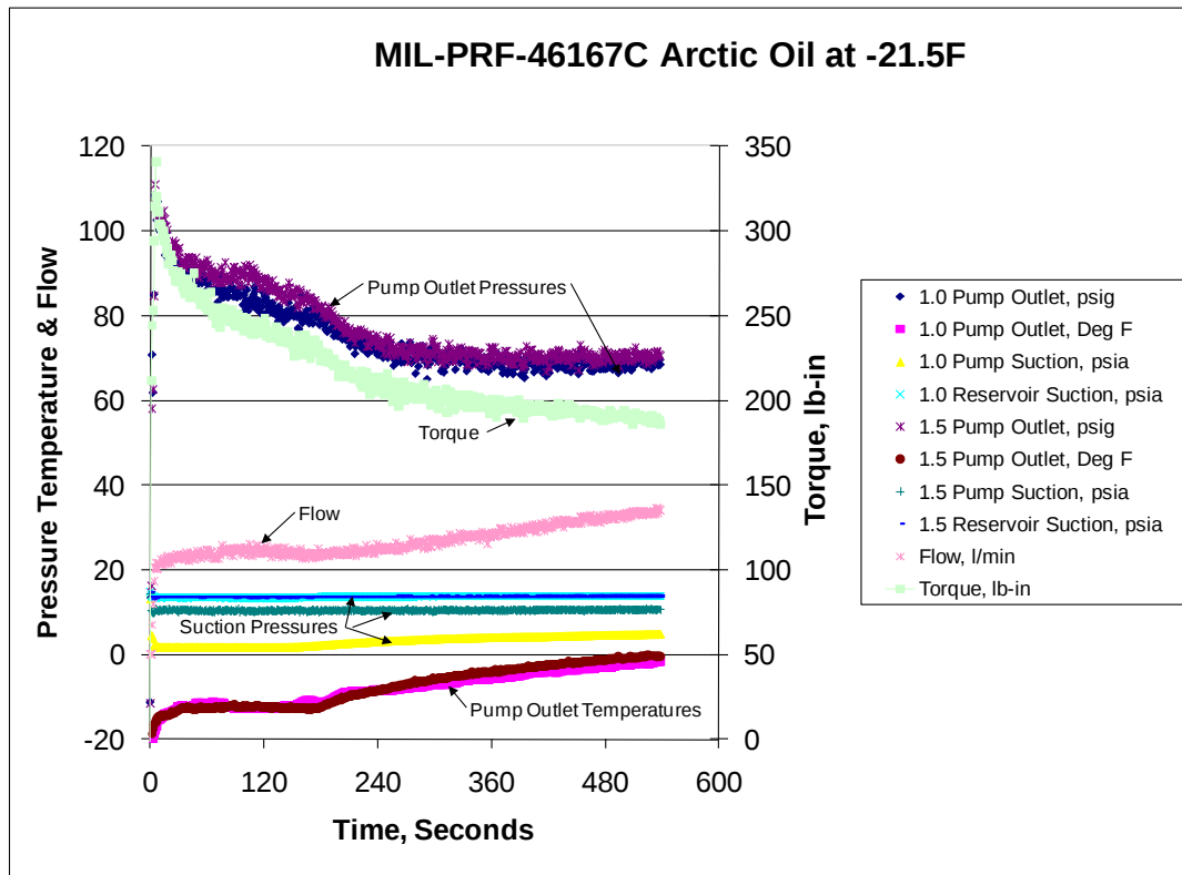
Figure 8. Typical Tandem Gear Pump Raw Data
