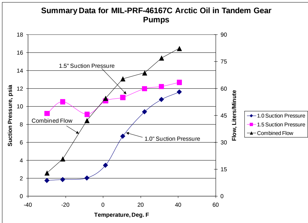
Figure 9. Summary Data for MIL-PRF-46167C Arctic Oil in Tandem Gear Pumps
