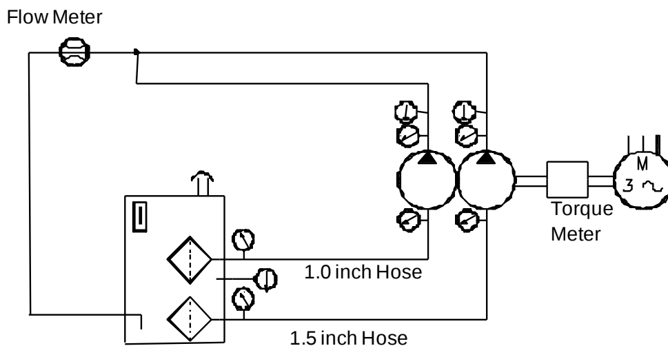
Figure 3. Fixed Displacement Tandem Pump Hydraulic Schematic
