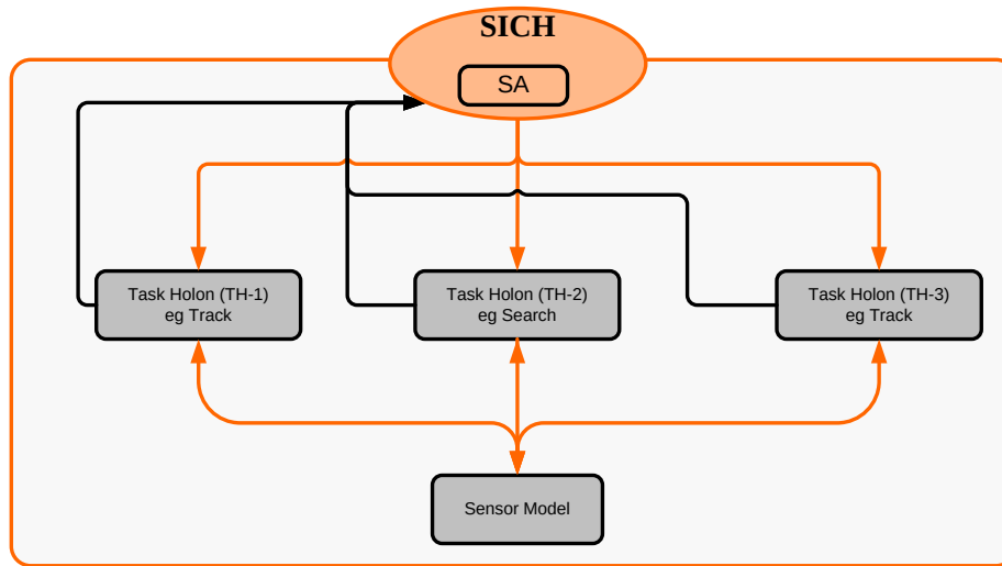
Figure 8: Sensor-level holon
