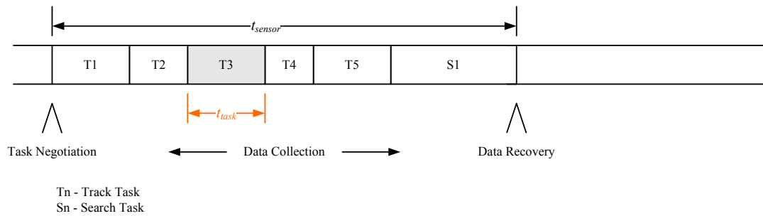
Figure 9: Scheduling within sensor control period
