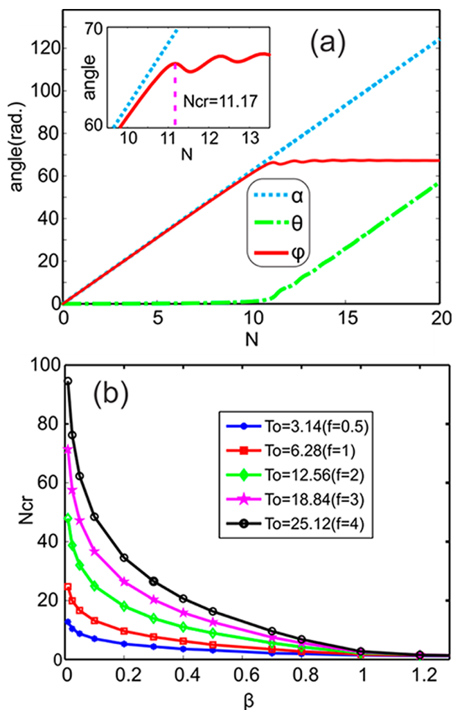
Figure 2. (a) Numerical solutions for \varphi , \alpha , and \theta as functions of the number of turns, N = tf , of a nanorod. The inset shows oscillating behavior of a nanorod which is about to stop its rotation after N_{cr} \sim 11 revolutions. (b) Dependence of the critical number of turns of a nanorod on parameter \beta .
