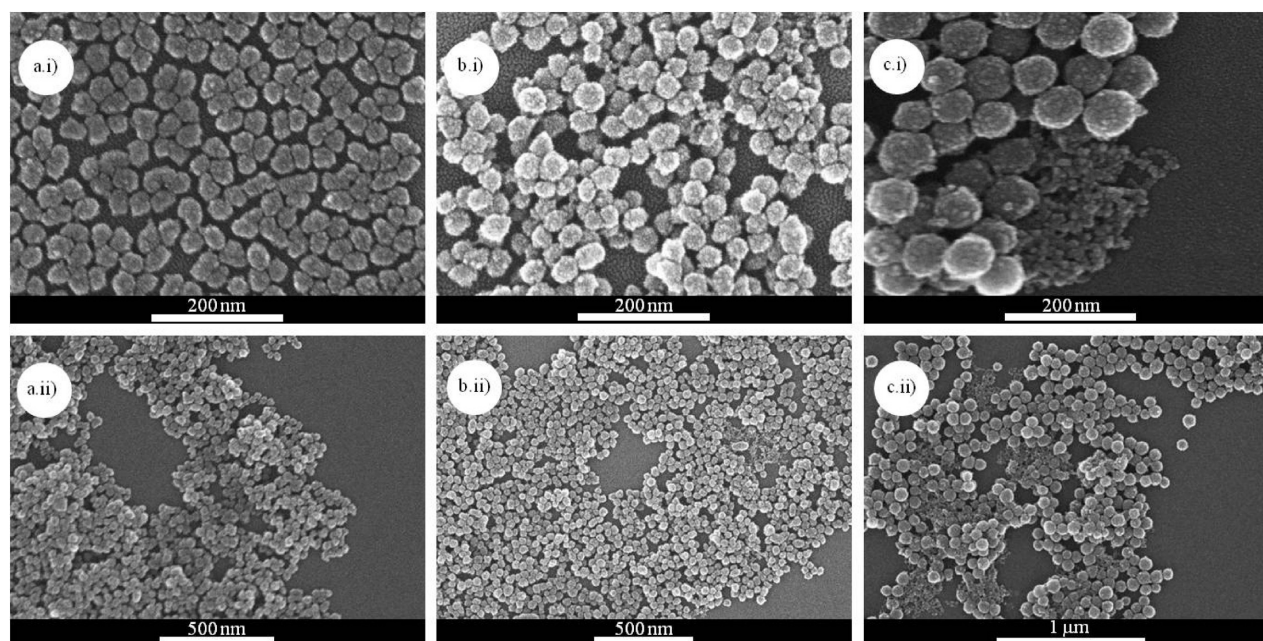
Figure 5. SEM images of SiO 2 NPs grown by time dependent reactions. NP diameters are (a) 29 \pm 6 nm, (b) 40 \pm 5 nm, and (c) 72 \pm 7 nm. SiO 2 NPs grown with shorter reaction times ( \leq 30 s) are irregular in shape and have rough surfaces.
