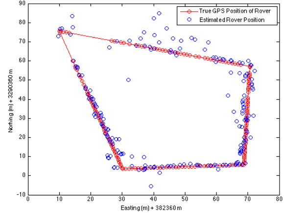
Figure 9: Result from Manual Test Using Aerial Image 2
