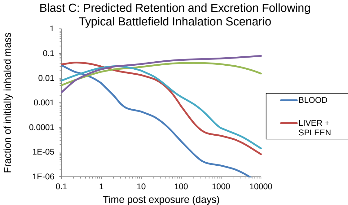
Figure 15. Biokinetic trends predicted by chemIMBA for a typical battlefield inhalation scenario following a detonation of an explosive containing Blast C formulation
