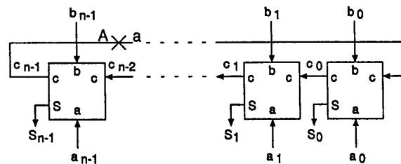
Figure 1. 1's complement adder circuit
