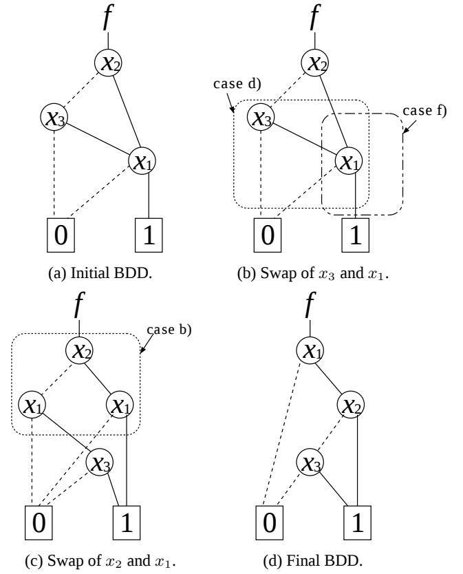
Figure 5.1. Example of sifting on BDD.
