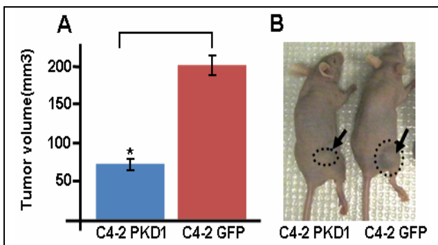
Figure 14: PKD1 expression suppresses prostate tumor growth in xenograft mouse model. To determine if PKD1 suppresses tumorigenesis in-vivo , PKD1 overexpressing C4-2-GFP-PKD1 cells and control C4-2-GFP cells ( 10 \times 10^6 ) were injected subcutaneously (s.c) into the flank of athymic nude mice. C4-2 cells expressing PKD1 formed significantly smaller tumors compared to control C4-2-GFP cells.
