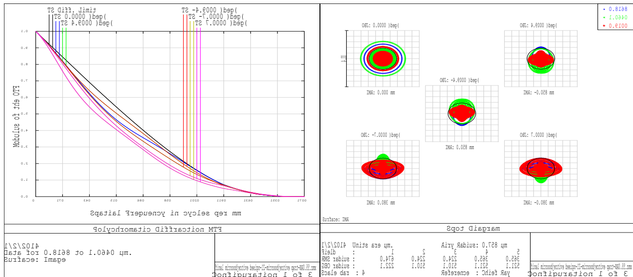
Figure 10: As-built image performance of the micro-objective system. (A) MTF performance; (B) spot diagram.
