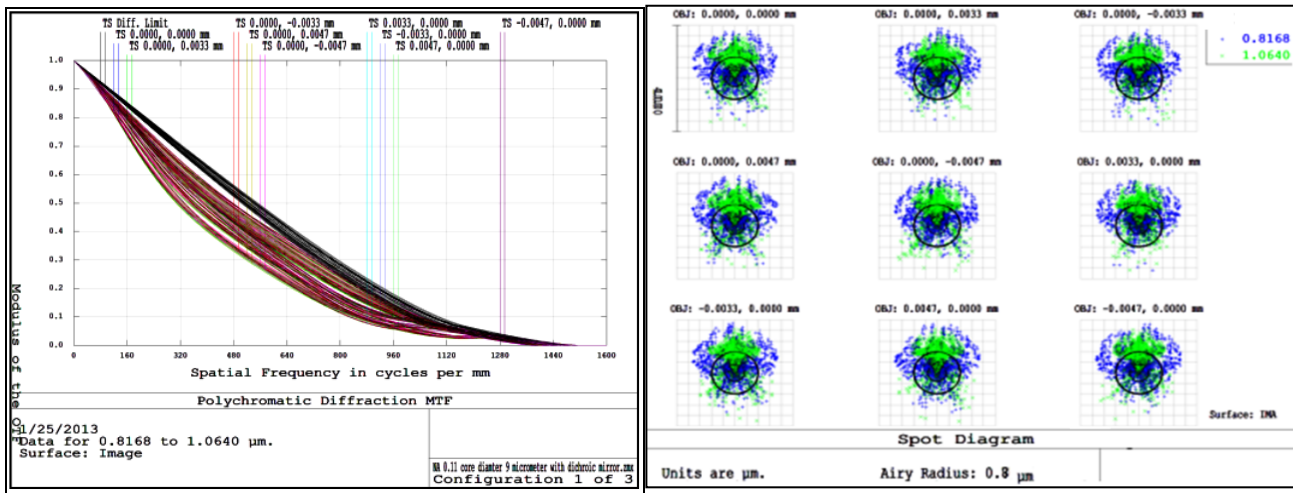
Figure 8: As-built image performance of CARS microendoscope probe. (A) MTF performance; (B) spot diameter at different FOVs.
