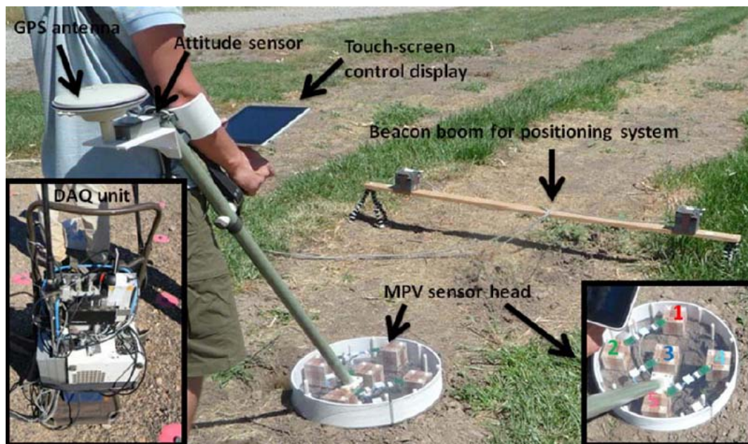
Figure 7-4 – photograph of the MPV sensor and beacon positioning system. The sensor head weighs 12 pounds and the backpack-mounted acquisition computer and batteries weigh 35-40 pounds.
