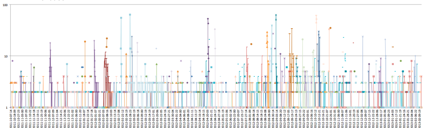
Figure 3.: KBA 2013's 141 query entities and their vital document counts per hour. Several spikes are visible. Most spikes are echos in the blogosphere that reverberate after a single event, which is often characterized by changes to a few strongly typed entity attributes or relationships, such as death or the breakdown of a corporate or spousal relationship.
