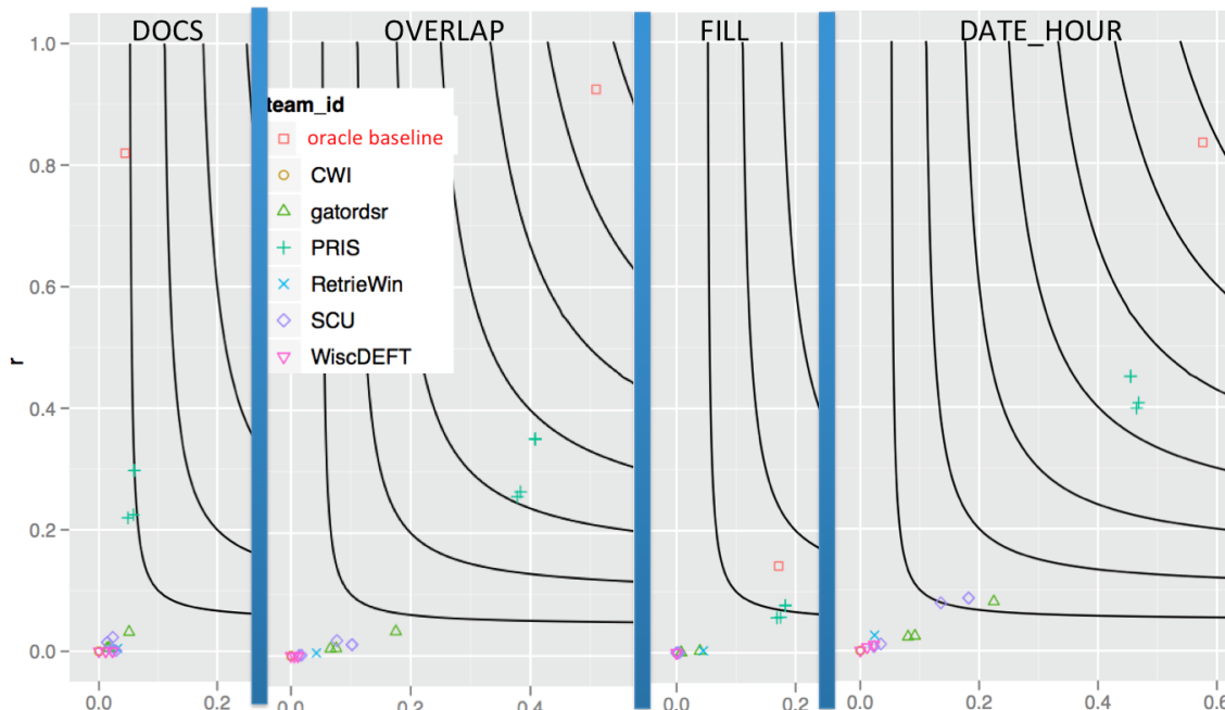
Figure 7: macro-averaged recall versus precision with curves of constant F_1 for the four stages of SSF scoring. Only the first level (DOCS) is a valid comparison across systems, because the subsequent stages only consider an individual system’s true positives from the previous stage. The high-recall of the oracle baseline is accomplished by asserting all possible slot types for every document that matches the surface form name of an entity. See the implementation of the baseline system in the github repository for the “toy_kba_algorithm.py”
