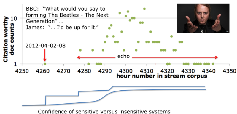
Figure 6: As an example, consider James McCartney, son of Paul McCartney, who confirmed in a BBC interview that he might start a new band called “Beatles II” or “The Beatles -- The Next Generation.” The large spike of echoes that resulted all contain redundant information. A good SSF system detects the change early. Example text: “Nothing may be sacred after all: Sir Paul McCartney’s son James is interested in starting a second-generation Beatles band with John Lennon’s son Sean, George Harrison’s son Dhani and Ringo Starr’s son Zak.”
