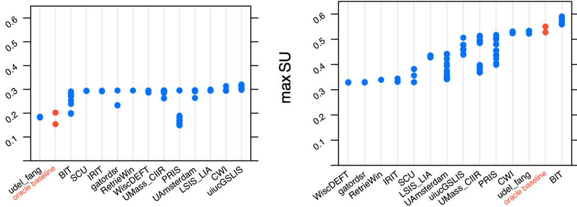
Figure 4: Official scores using “vital” and “vital+useful” as the classification objective. The red points represent the oracle baseline system that used a hand-picked set of names to select a high-recall set of documents.
