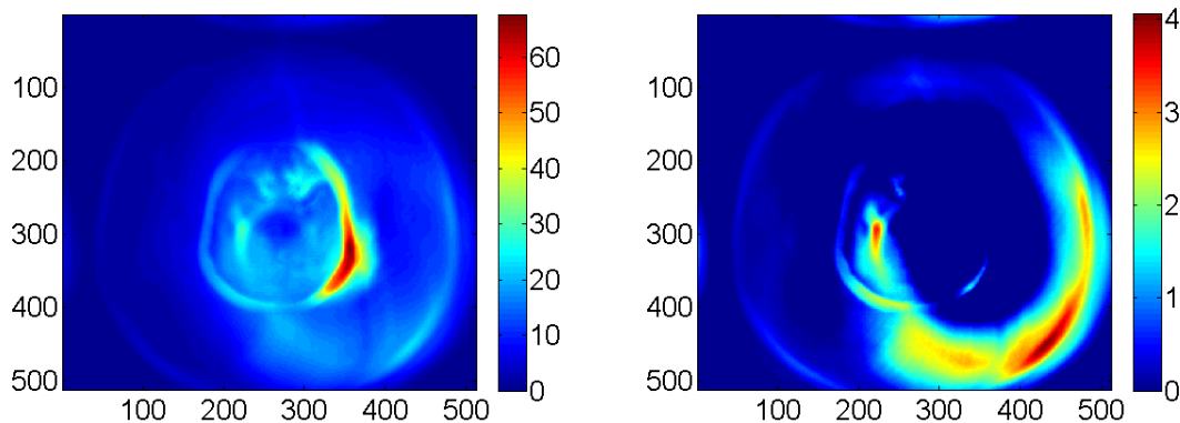
Figure 4.15: (L) Unfiltered reconstruction of the textbook cover at 435 nm focus. (R) Filtered reconstruction of the textbook at 435 nm in focus. The filter parameter \mu was 5. The filter deleted a lot of the energy in the scene, including where unfiltered intensities were the highest.
