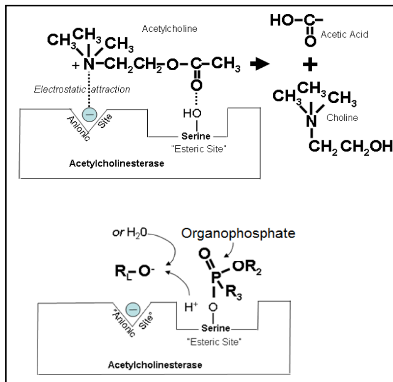
Figure 2: Normal Acetylcholine Hydrolysis and Inhibition of AChE by OP
