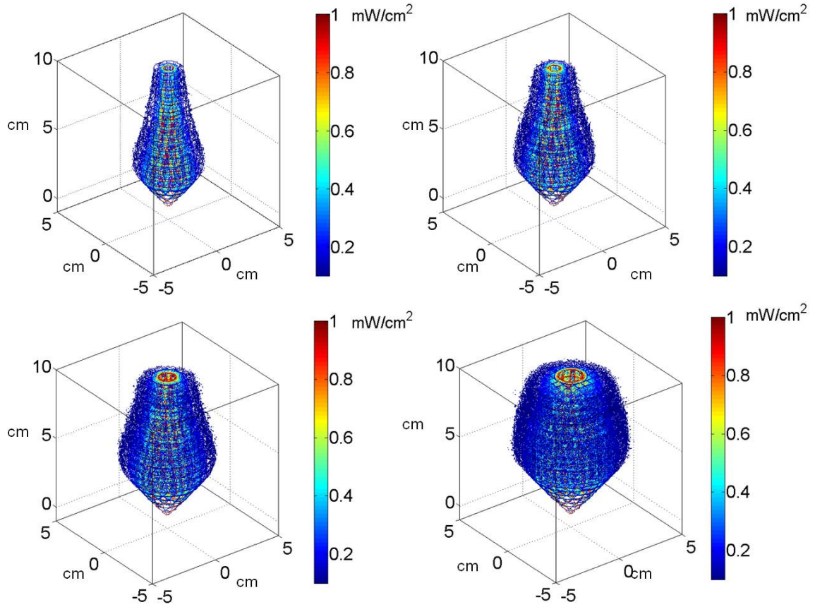
Figure 30: Single Bulb 0.1 to 1 mW/cm 2 , Top Left 180 \mu\text{W} , Top Right 300 \mu\text{W} , Bottom Left 567 \mu\text{W} , Bottom Right 1200 \mu\text{W}
