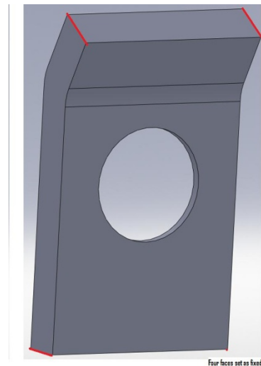
FIGURE 7: FOUR EDGES SET AS "FIXED"
