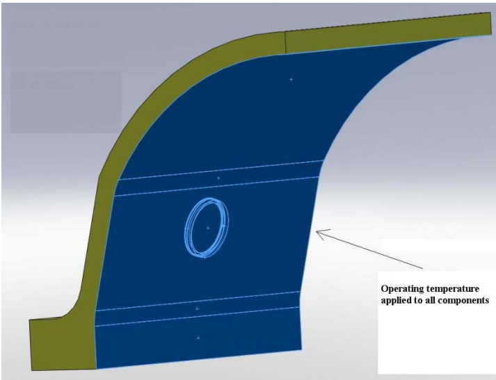
FIGURE 14: FEA THERMAL LOAD
