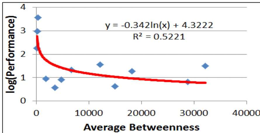
Figure 60 - Log-10 of the performance improvement of the incremental betweenness centrality algorithm vs. Average betweenness centrality.
