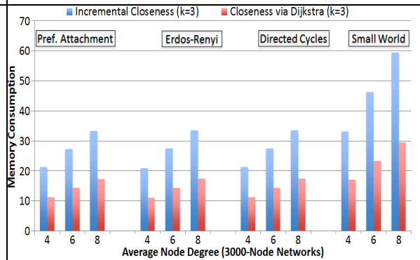
Figure 33 - Memory statistics incremental closeness algorithm with the Dijkstra's algorithm for closeness. Both are bounded by k = 3 .
