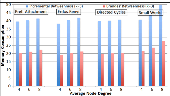
Figure 39 - Memory statistics comparing the incremental betweenness algorithm with the Brandes' algorithm. Both are bounded by k = 3 .
