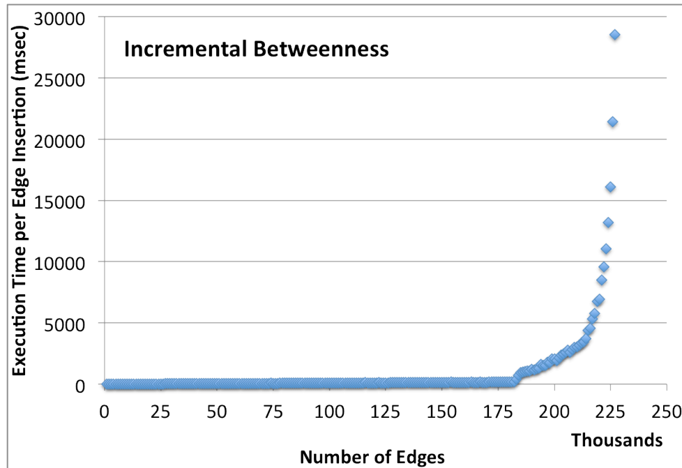
Figure 43 - Incremental betweenness centrality algorithm execution time per edge insertion in milliseconds versus the number of edges inserted. The numbers of edges are represented in thousands, where '200' on the x -axis represents 200,000 edges. The execution time per edge insertion is given in milliseconds, 30,000 represents the 30 seconds.
