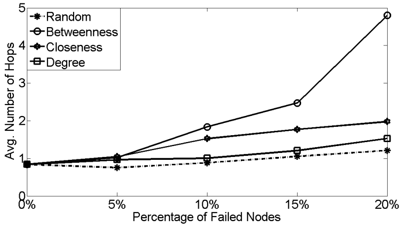
Figure 12 - Increase in average number of hops as top ranked nodes are progressively removed from a 200-node wireless mesh network topology.
