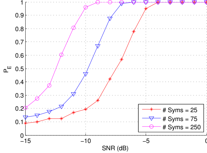
Figure 3.6: Probability of correct estimation of sampling rate.
