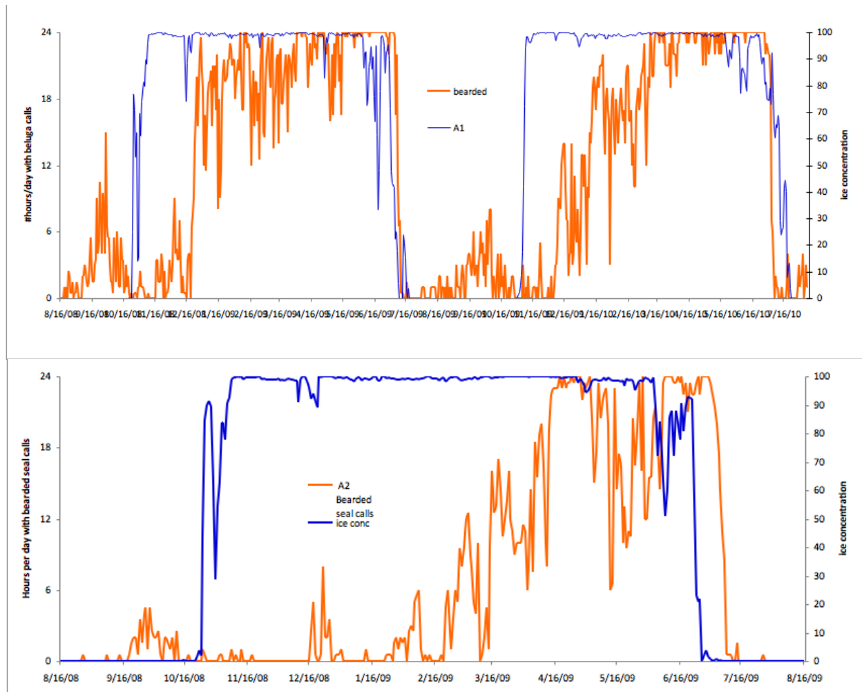
Figure 6. Number of hours per day with bearded seal call detections (orange line) and ice concentration (blue line) within 30 km of mooring sites. Upper panel: Mooring site A1, 2008-2010. Lower panel: Mooring site A2, 2008-2009. Detection of bearded seal calls was strongly associated with ice cover, increasing dramatically in late December and early January and being the dominant signal when ice cover approached 100%. Bearded seal calls decreased abruptly with reduction in sea ice.
