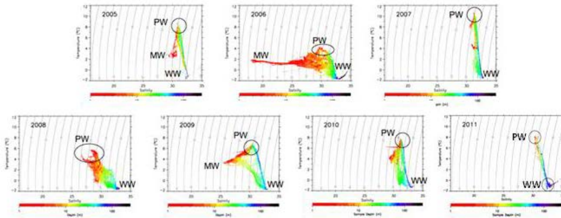
Figure 2. Temperature-salinity plots of each year's CTD data. Representative water masses are Pacific Water (PW), Winter Water (WW), and sea ice Melt Water (MW). Curved lines are isopycnals (constant \sigma_t ). Color indicates water depth at each data location. Highest Pacific Water temperature ( \sim 12^\circ\text{C} ) was observed in 2007; lowest Pacific Water temperature ( \sim 4^\circ\text{C} ) was observed in 2006, with the greatest amount of sea ice Melt Water also seen in that year.
