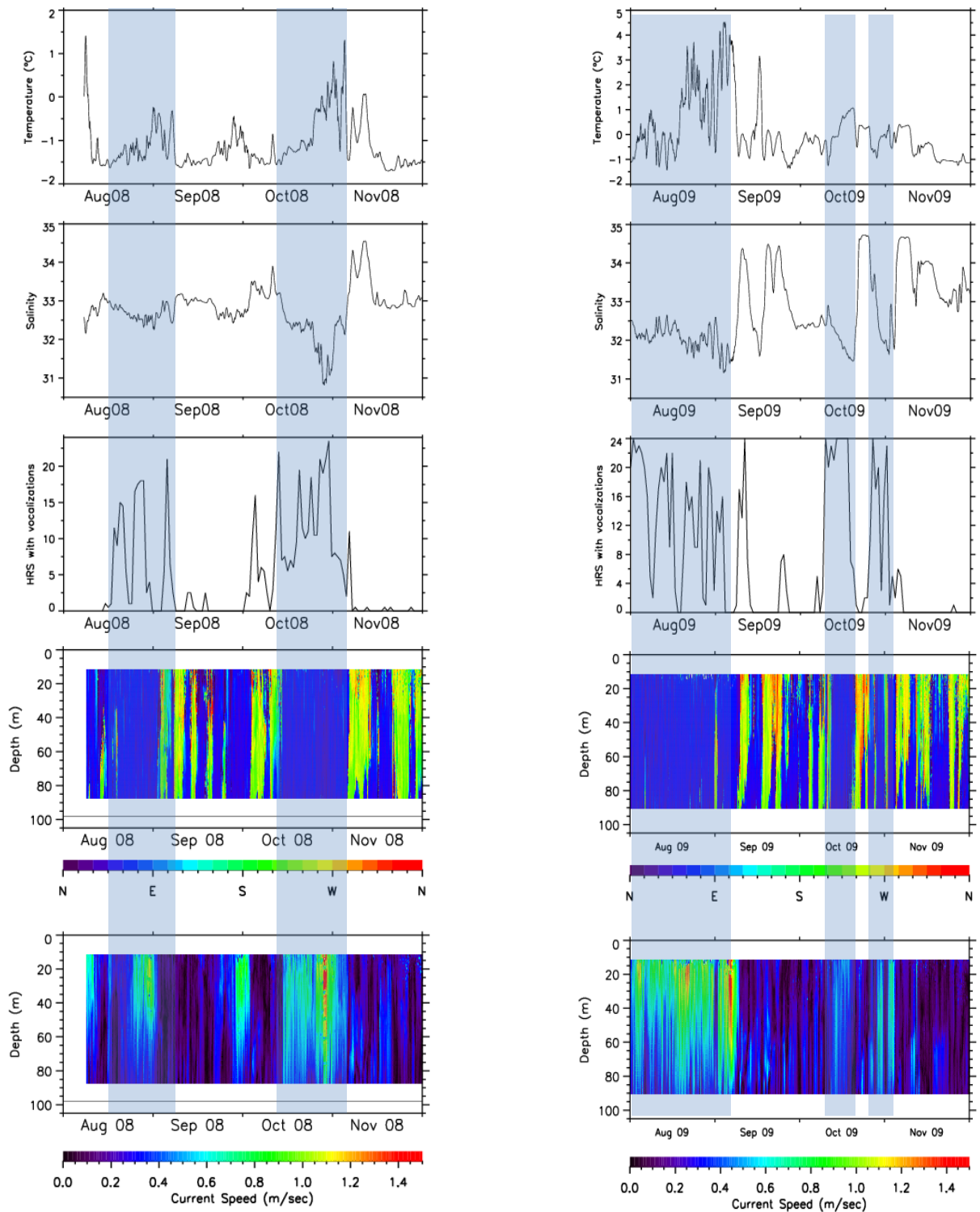
Figure 7. Associations between near-bottom (88 m) water temperature and salinity (upper two panels), occurrence of beluga whale vocalizations (middle panel) and water column velocity (speed and direction) at the A1 mooring during late summer-early fall of 2008 (left) and 2009 (right). Beluga calls were more frequent when the Alaska Coastal Current (high, northeastward velocity) containing Alaska Coastal Water (warmer, fresher) was present over the mooring (noted by blue shading).
