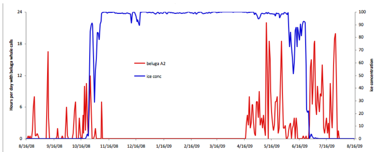
Figure 5. Number of hours per day with beluga whale call detections (red line) and ice concentration (blue line) within 30 km of mooring sites. Upper panel: Mooring site A1, 2008-2010. Lower panel: Mooring site A2, 2008-2009. Beluga whale call detections decreased in fall as ice cover increased but increased in both springs while ice cover was still extensive.
