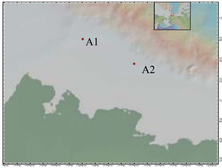
Figure 1. Locations (red circles) of moorings along the Beaufort Shelf break recovered during the 2010 Healy cruise.
