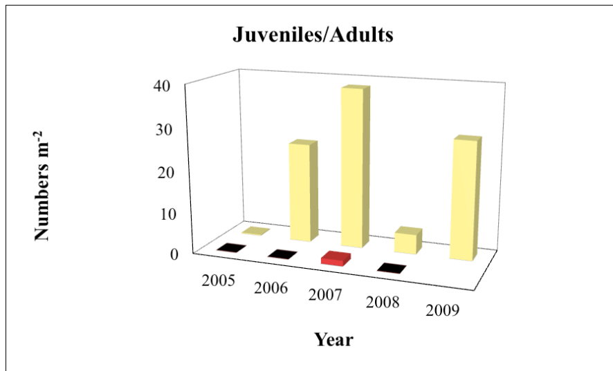
Figure 3. Abundance of bowhead whale prey (juvenile and adult euphausiids) on the shelf near Barrow following an upwelling/concentrating event (yellow) and before such an event or after the relaxation of the concentrating mechanism (red). Not all conditions were sampled in all years. Elevated concentrations of whale prey were observed on the shelf after upwelling east winds were followed by low or south winds.
