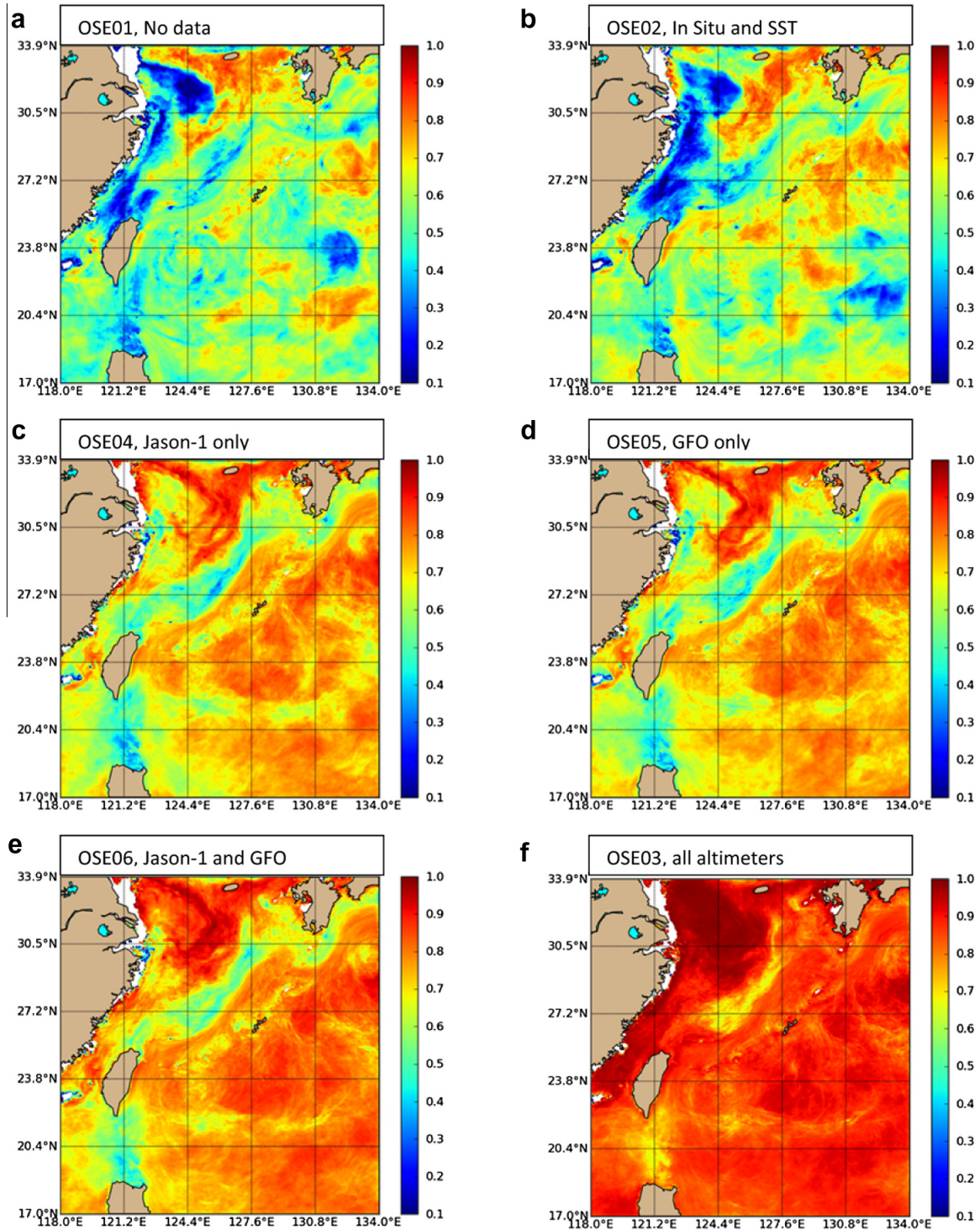
Fig. 10. The temporal correlation of MLD from the nature run and the OSEs constructed at each grid point using time series from which a 2 month boxcar filter has been applied and subtracted to remove long period variations. The results indicate increased skill as the number of altimeters increases as well as some spatial structure due to local processes affecting the skill. The correlations for OSEs with no data assimilate (a), all in situ data except altimeter (b), all in situ data with only Jason-1 altimetry (c), all in situ data with only GFO altimetry (d), all in situ data with only Jason-1 and GFO altimetry (e) and all in situ data with all altimeters (f) are shown.
