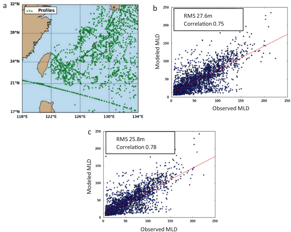
Fig. 4. Evaluation of the nature run MLD performance is made by comparison to in situ profile data during the experiment time period. The data locations are relatively randomly distributed with the exception of some ship of opportunity tracks (a). The model is sampled at the same times and locations. The scatterplots of the model 24 h forecast prior to the data being assimilated (b) and the model hindcast after the data have been assimilated (c) with the observed MLD indicate moderate skill in predicting the MLD. For the MLD prior to assimilation of data, the RMS error is about 27.6 m with a correlation coefficient of 0.75, while the RMS error after assimilation is smaller at about 25.8 m with a slightly higher correlation coefficient of 0.78. Assimilation, in general, does not make a very large correction day-to-day.
