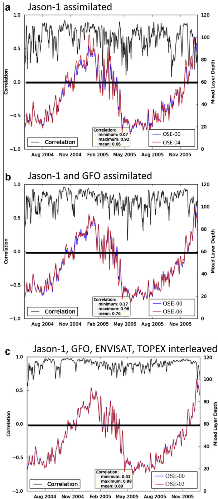
Fig. 9. MLD from the nature run is compared to MLD from several OSEs for the subdomain (20–24° N and 123–127° E) used in Fig. 6. The blue line is nature run MLD averaged over the subdomain and red line is the OSE MLD averaged over the subdomain. The seasonal cycle of MLD is apparent in all OSEs. The black line is the MLD correlation coefficient between the nature run and OSE over the subdomain. The minimum, maximum and time-averaged correlation coefficient are listed at the bottom of each plot. With one altimeter (a) the correlation is significant though frequently drops below the significance level of 0.62. The rate at which the correlation is below the significance level decreases with 2 satellite altimeter (b). Assimilating all 4 available altimeters results in the correlation always above the significance level (c).
