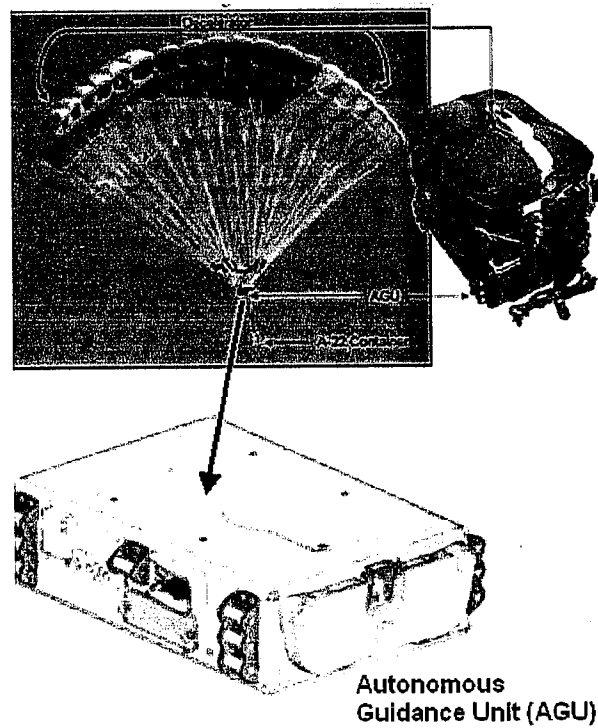
Figure 9: JPADS 2,400-pound Delivery System
