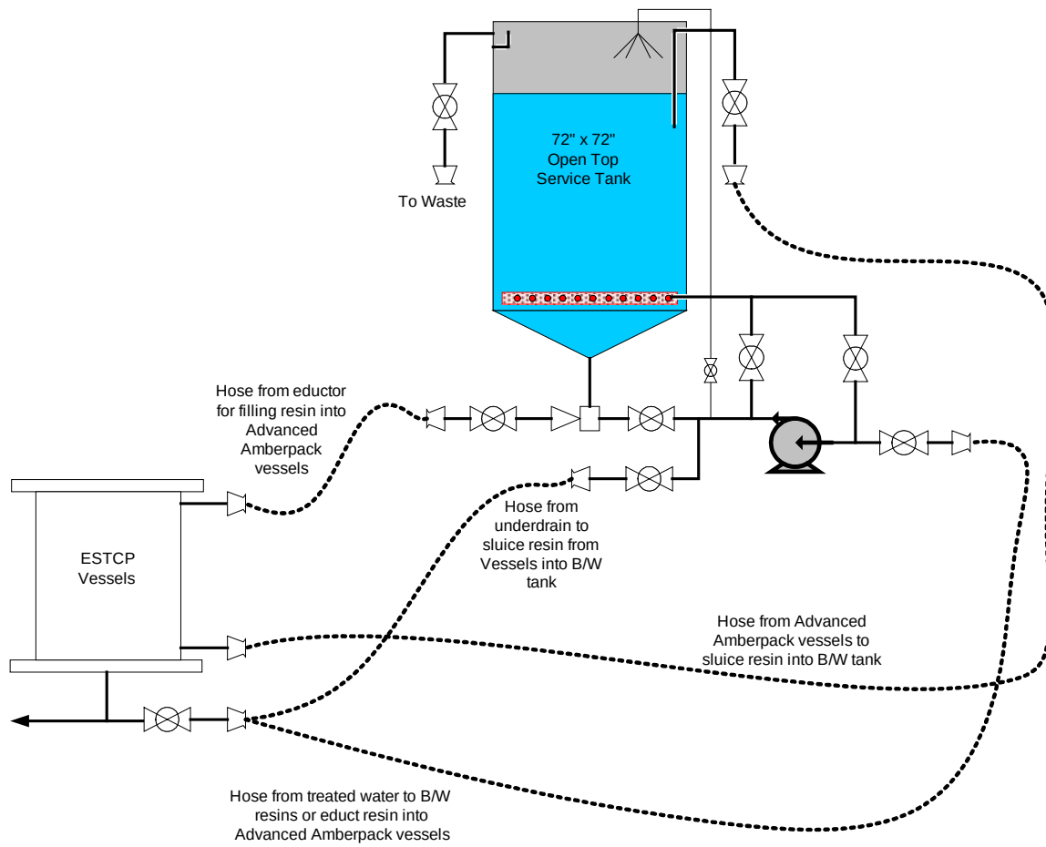
Figure 13. Process Flow Diagram for ESTCP Resin Loading and Service Vessel.
