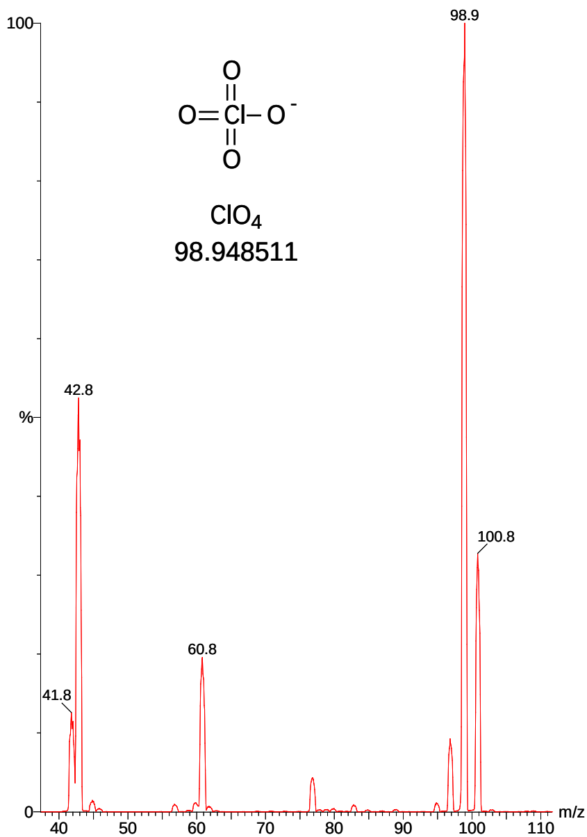
Figure 4. Mass spectrum of a 1 ppm perchlorate standard obtained by infusion.
