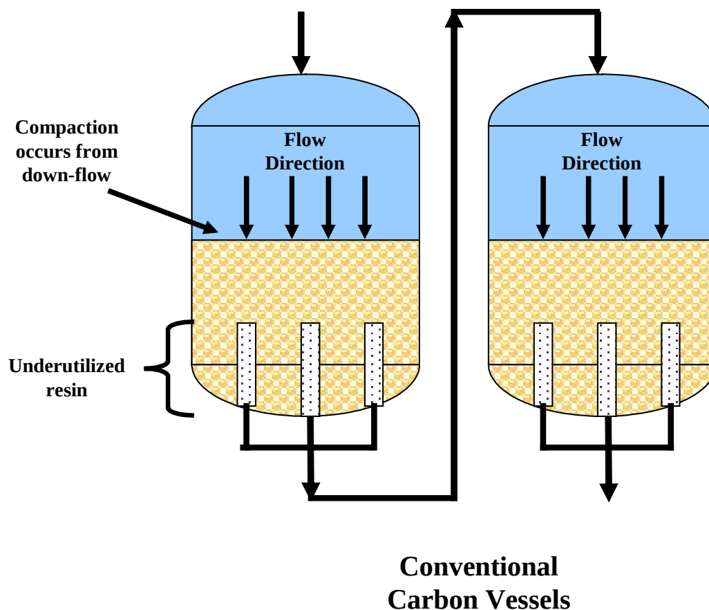
Figure 2. Typical Lead-Lag Carbon Vessel design
