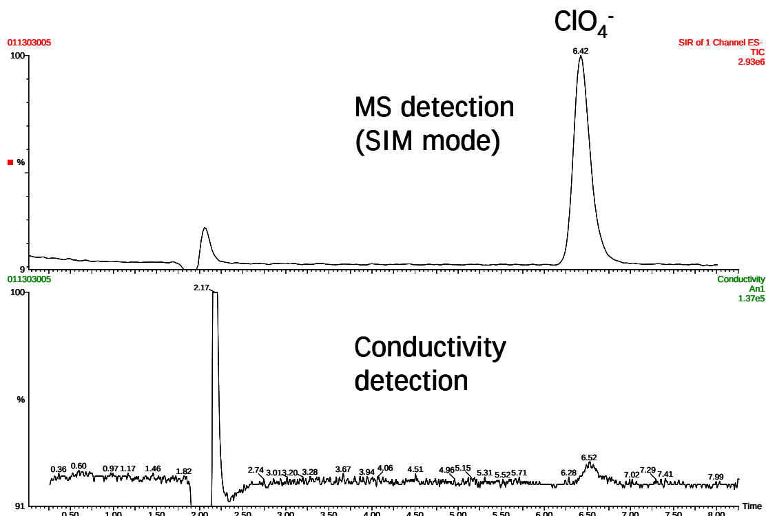
Figure 3. Separation of a 0.5 ppm perchlorate standard by mass spectrometry (top) and conductivity (bottom) detection modes.
