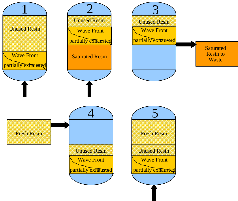
Figure 7. Resin exhaustion and replacement process for ESTCP demonstration project (up-flow water service).
