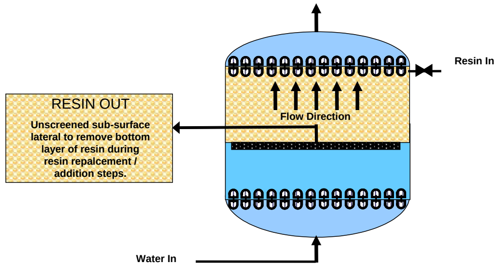
Figure 5a. Schematic of vessel for ESTCP demonstration project. Normal operation.
