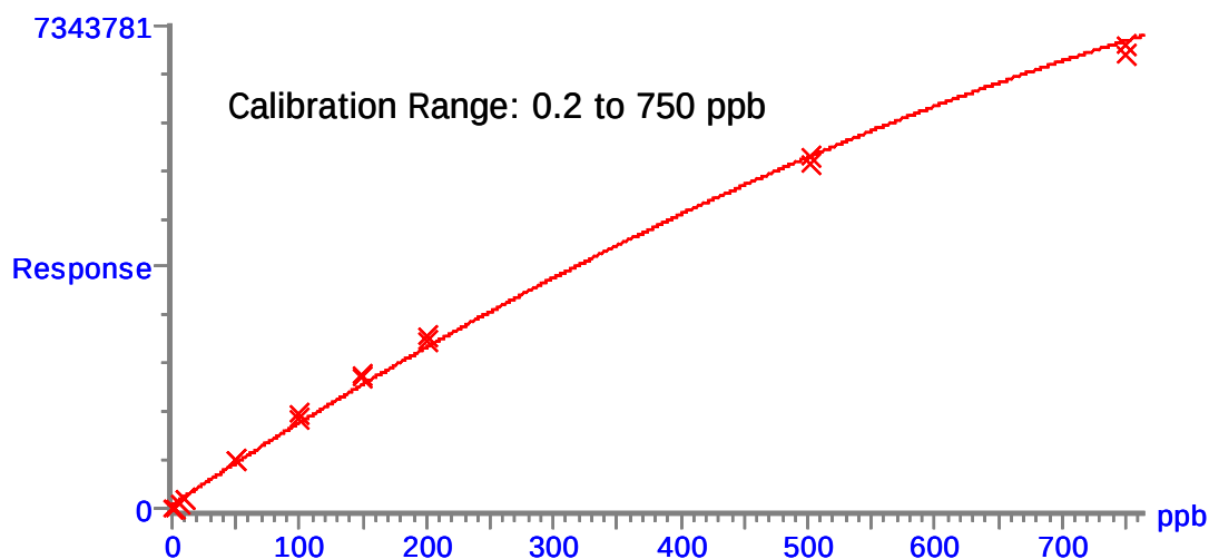
Figure 7. Calibration curve for perchlorate with mass spectrometry detection over a broad calibration range.
