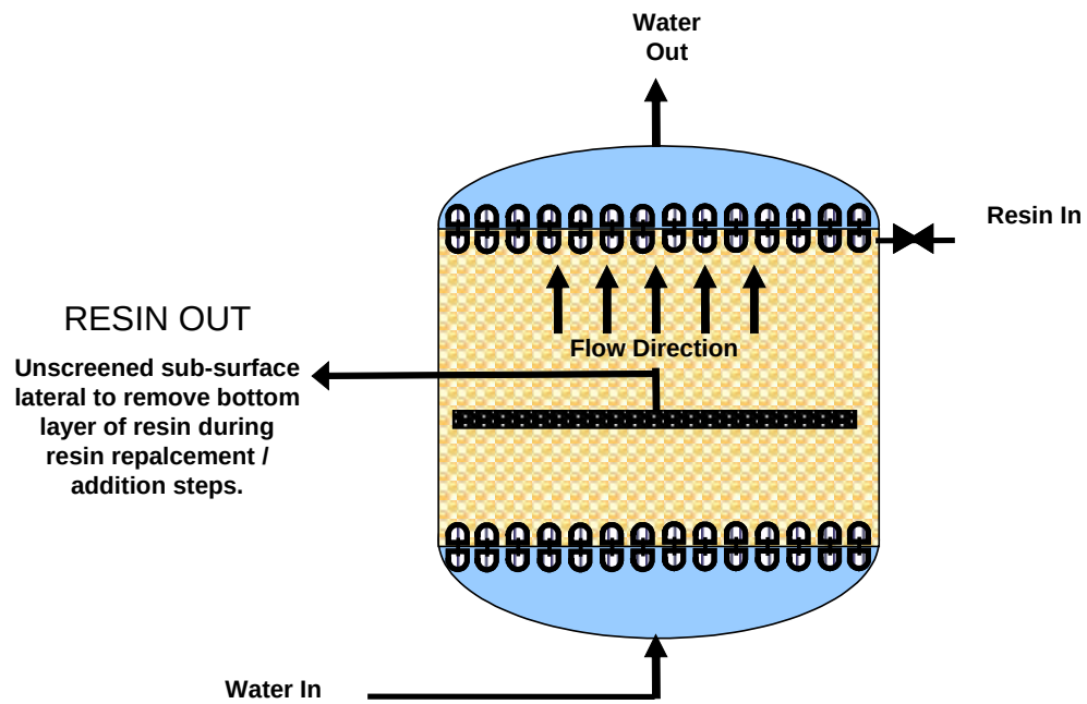
Figure 5b. Schematic of vessel for ESTCP demonstration project. Service mode.
