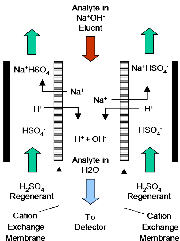
Figure 2. Schematic of suppressor used in anion exchange chromatography.
