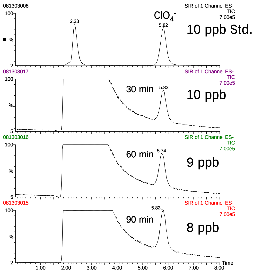
Figure 8. Separation of a 10 ppb perchlorate standard and three effluent samples (different collection times) that contain low ppb perchlorate levels in the presence of sulfate.
