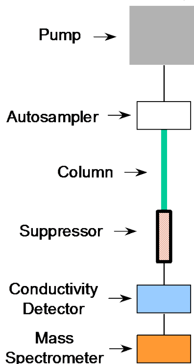
Figure 1. Schematic of IC/MS system.
