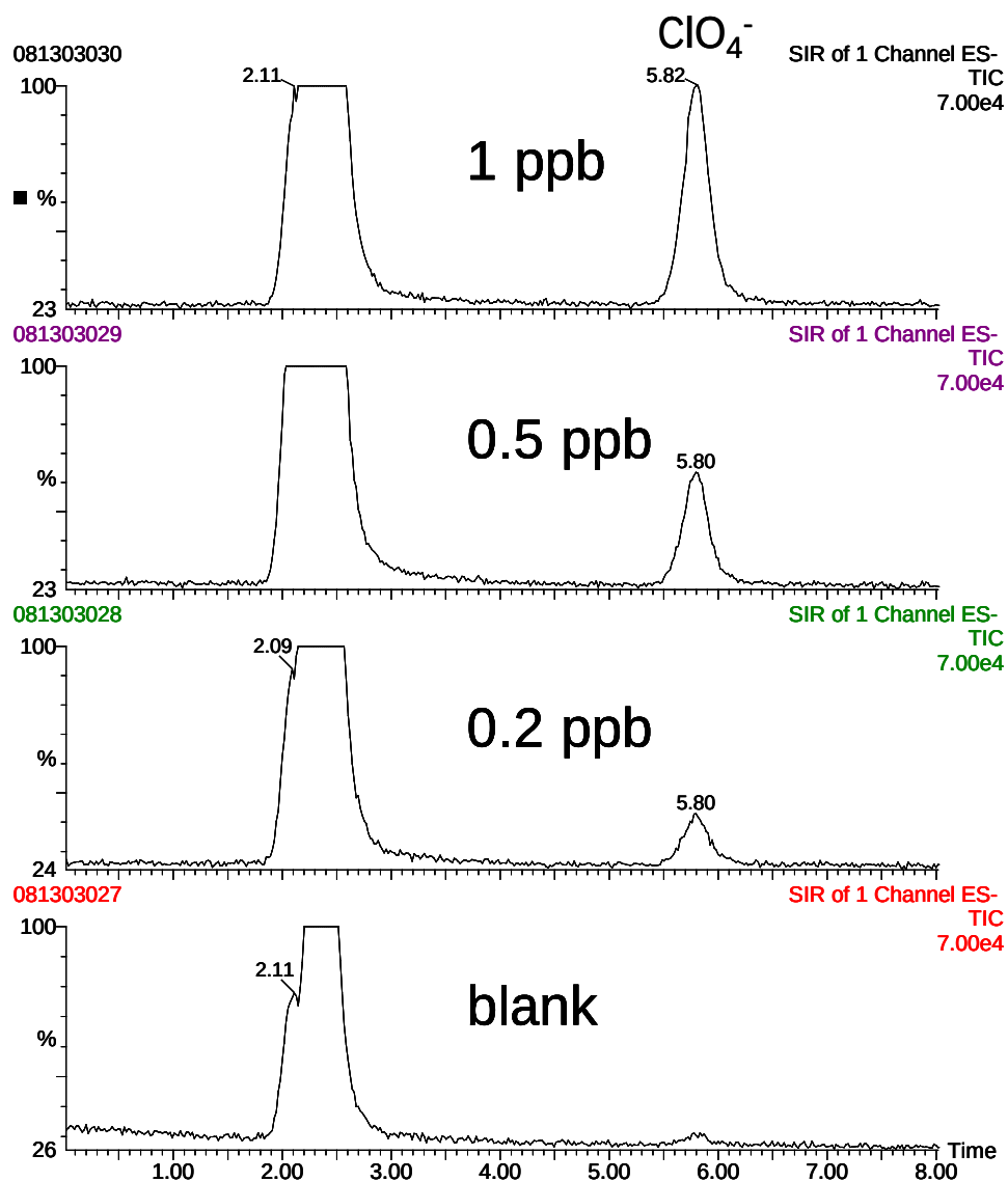
Figure 5. Separation of three low ppb perchlorate standards with mass spectrometry detection.
