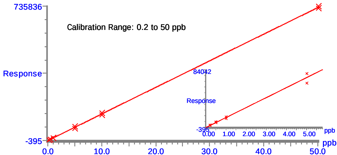
Figure 6. Calibration curve for perchlorate with mass spectrometry detection. Insert shows the linearity at low ppb levels.
