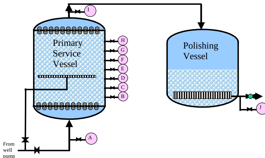
Figure E1. Relative Location of Sample Taps for ESTCP System.
