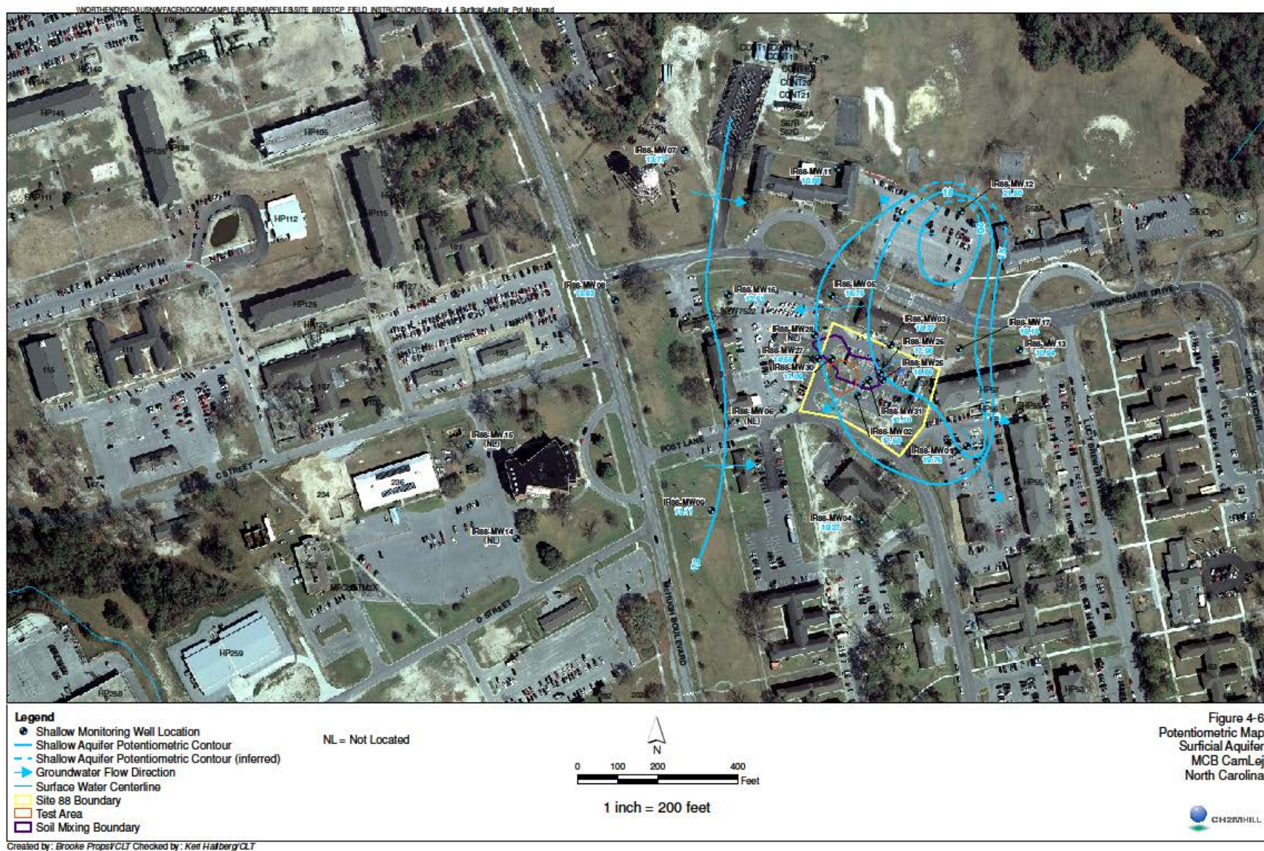
Figure A-6. Potentiometric map of the Surficial Aquifer
