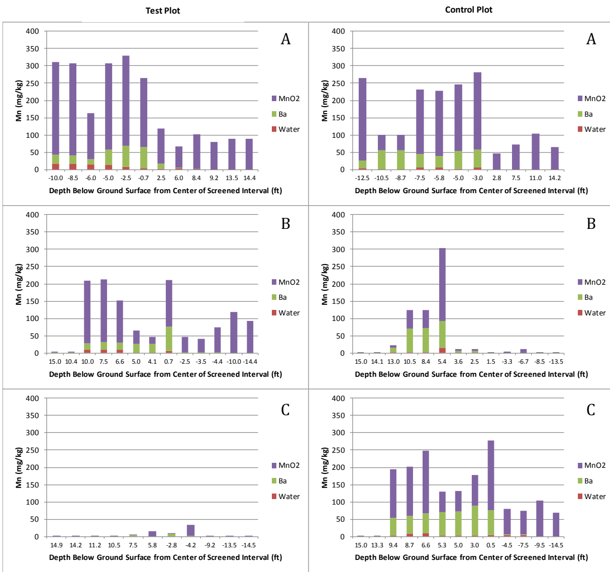
Figure 5-52. Manganese as water-extractable, Ba-extractable, and as MnO 2 for test and control plot cores collected one year post-treatment with respect to depth (relative to the center point of the screened interval). Charts designated (A) are for cores approximately 5 ft. from injection, (B) are approximately 10 ft. from injection, and (C) are approximately 15 ft. from injection.
