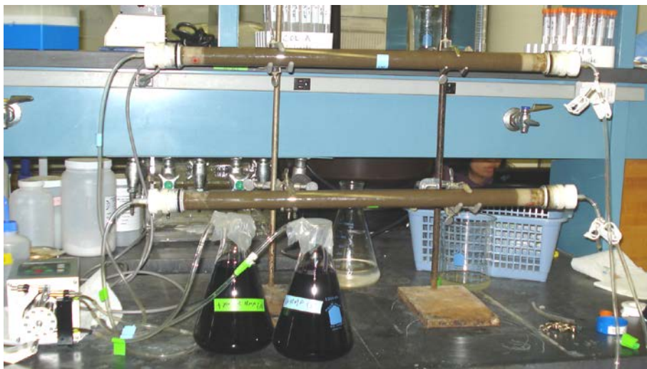
Figure 10. 1-D packed columns for evaluation of permanganate and SHMP transport through site porous media. The top column is permanganate-only and the bottom is permanganate + SHMP.
