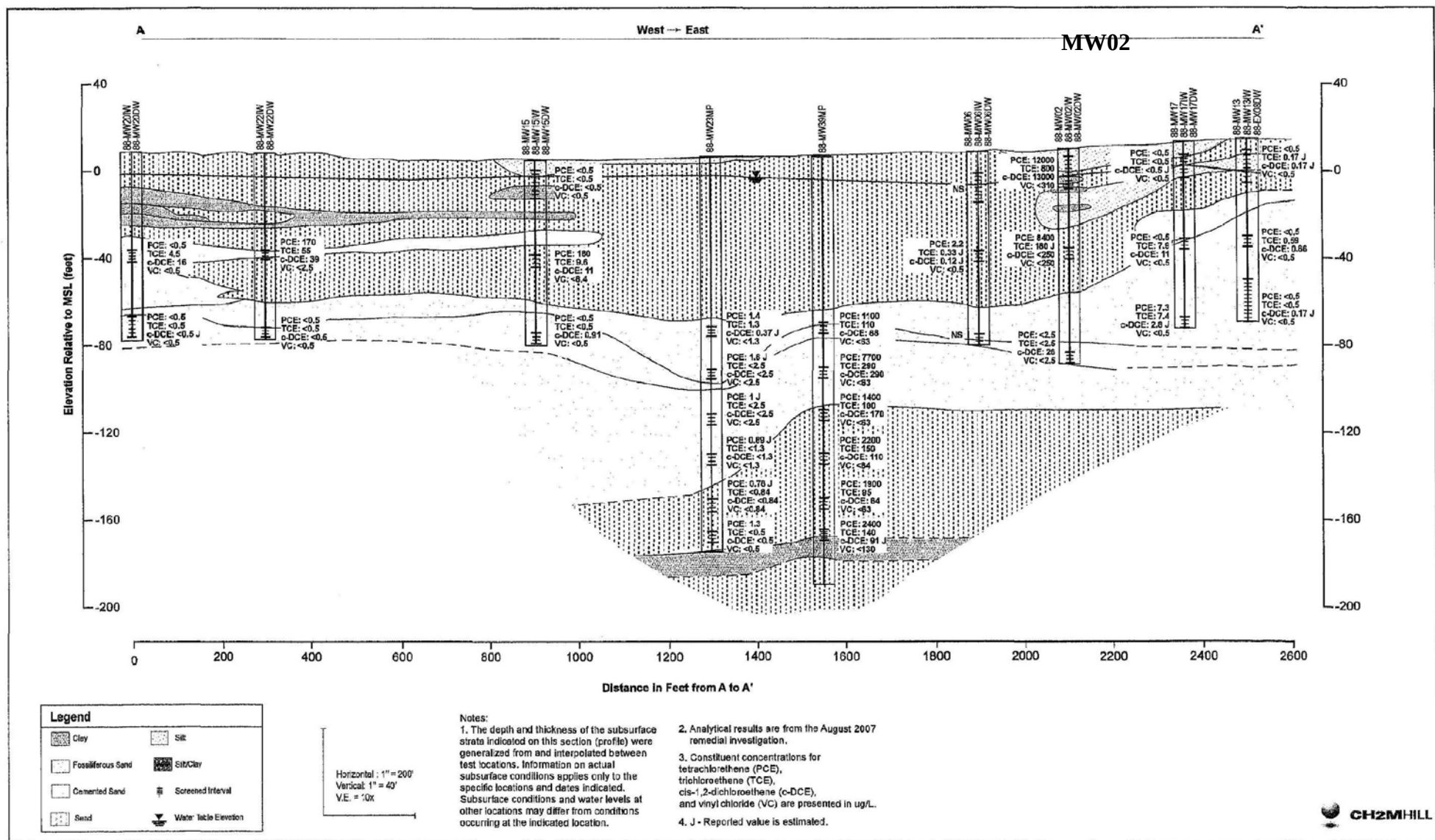
Figure 3. Cross-section A-A'
