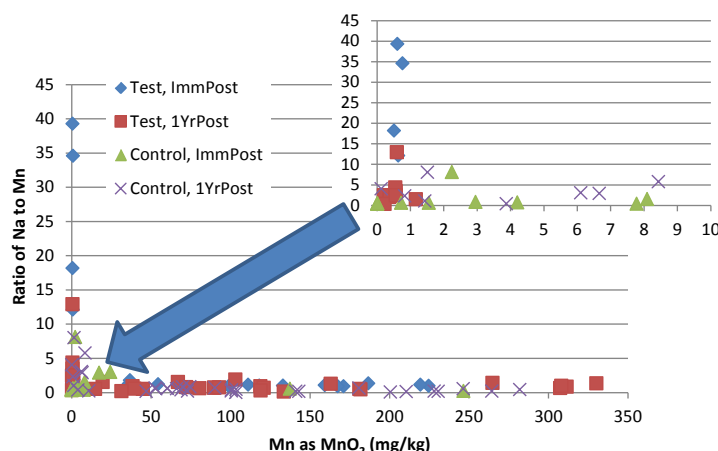
Figure 5-55. The ratio of Na to Mn with MnO 2 concentration for test and control plots immediately post-treatment (Test, ImmPost and Control, ImmPost, respectively) and 1 year post-treatment (Test, 1YrPost and Control, 1YrPost, respectively).
