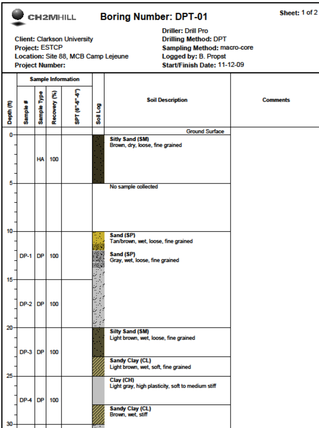
Figure 4-6. Boring Log for DPT01
