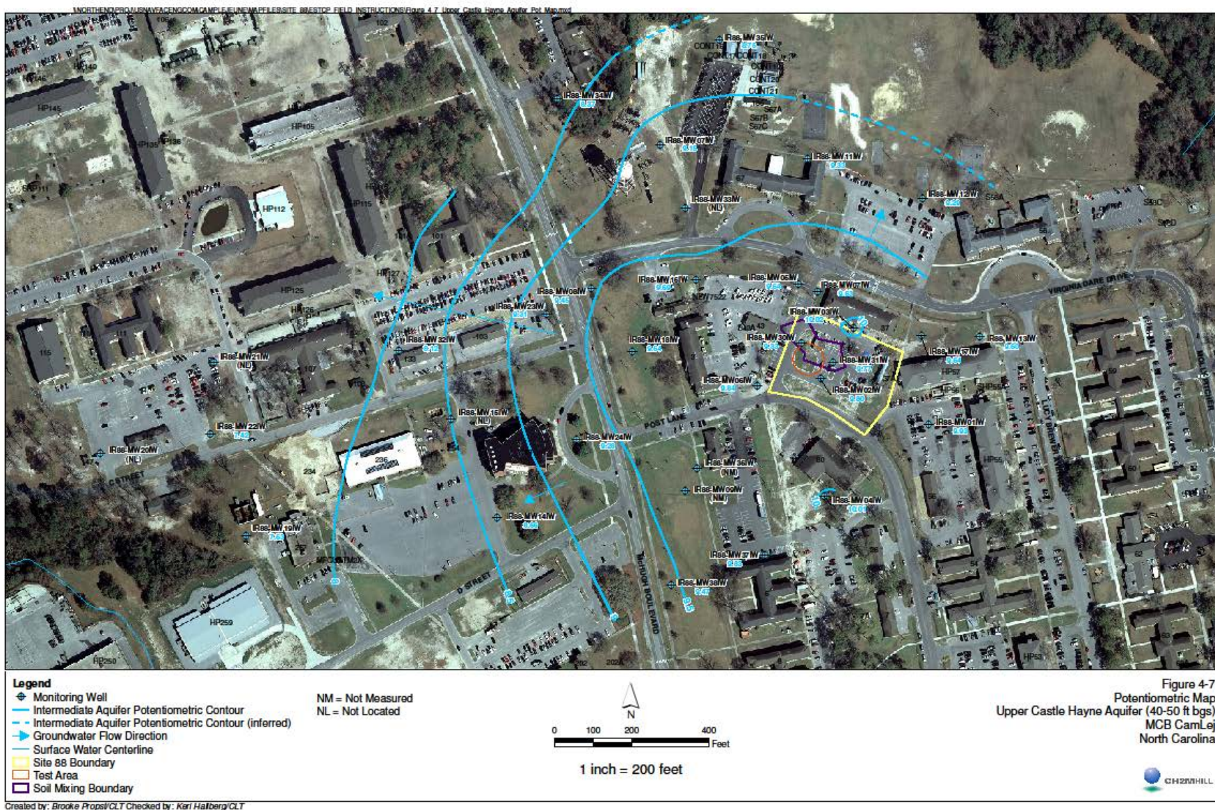
Figure A-7. Potentiometric map of the Upper Castle Hayne Aquifer
