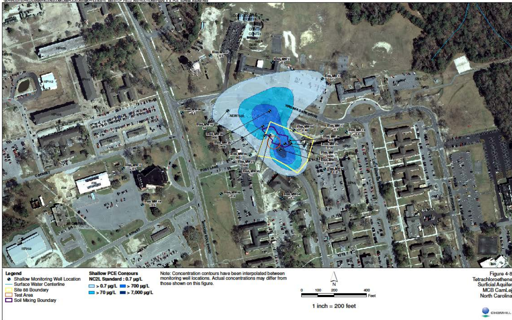
Figure A-8. PCE concentrations in the Surficial Aquifer (2007)
