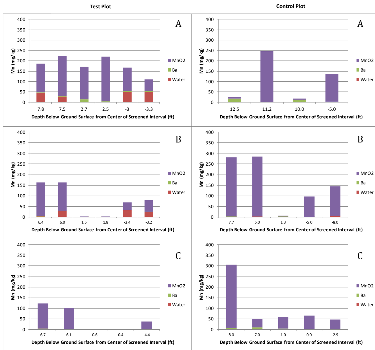
Figure 5-51. Manganese as water-extractable, Ba-extractable, and as MnO 2 for test and control plot cores collected immediately post-treatment with respect to depth (relative to the center point of the screened interval). Charts designated (A) are for cores approximately 5 ft. from injection, (B) are approximately 10 ft. from injection, and (C) are approximately 15 ft. from injection.
