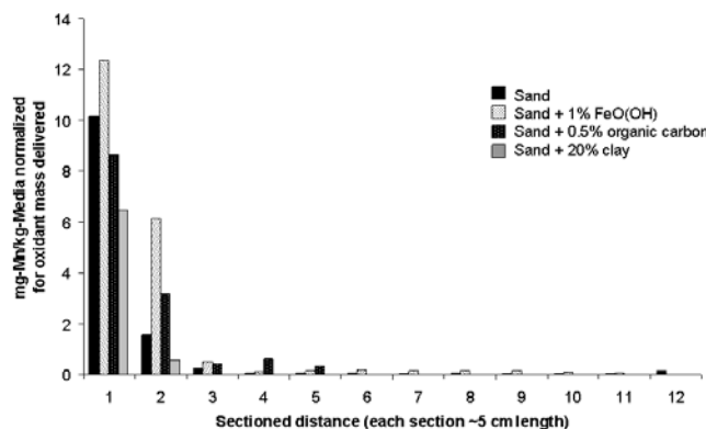
Figure 2-11. Mass of Mn (as \text{MnO}_2 ) per kg of media with distance from 1-D column influent. Each section is approximately 5 cm of column length. Results are normalized for the total mass of permanganate delivered to the column. Delivery mass differed for columns due to plugging and restricted flow in Sand + Goethite and Sand + Clay columns.
