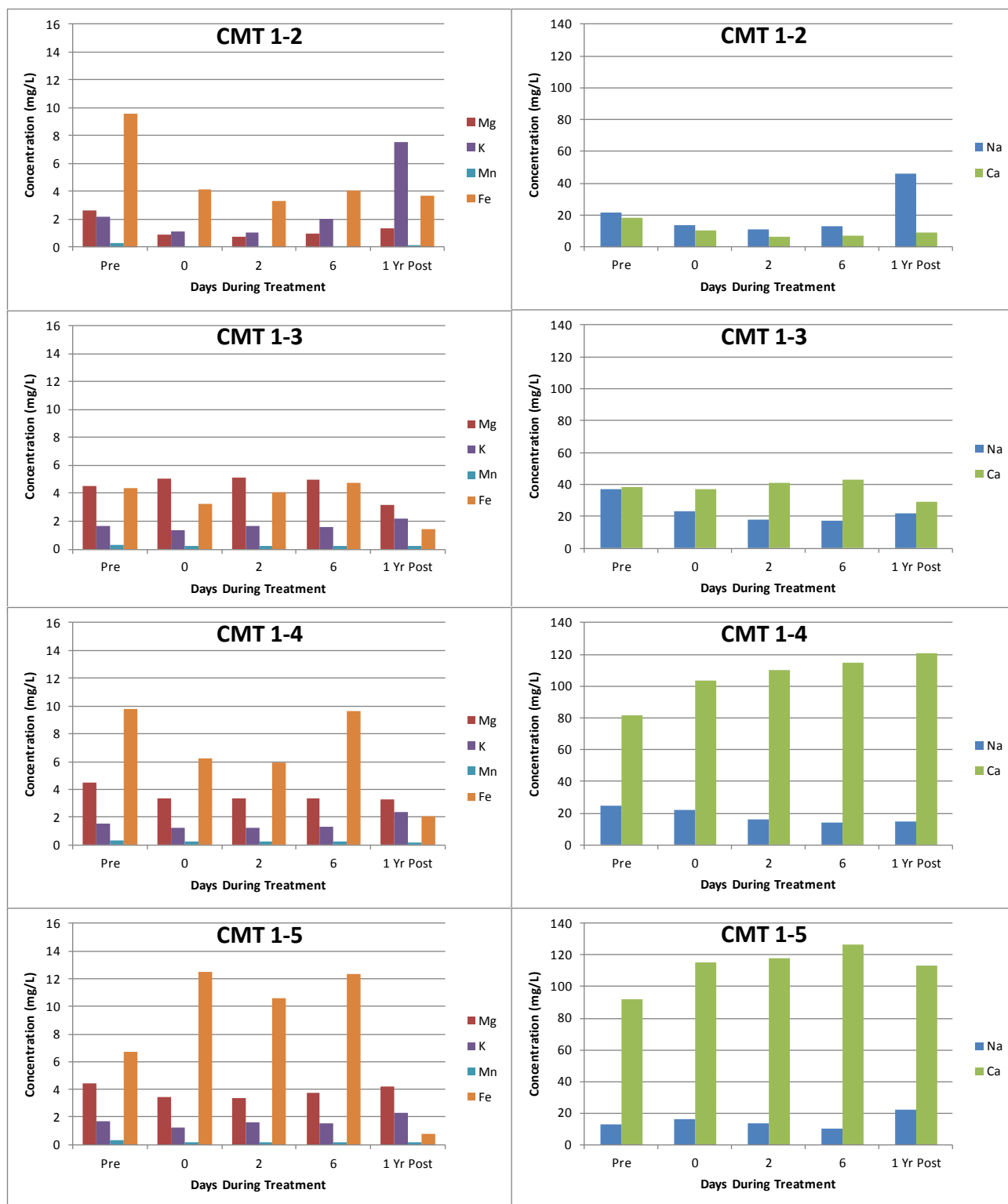
Figure 5-41. Concentrations (mg/L) of common cations measured in CMT 1 at each depth. Because of the data range, the left-hand side presents Mg, K, Mn, and Fe data, and the right-hand side presents Na and Ca.
