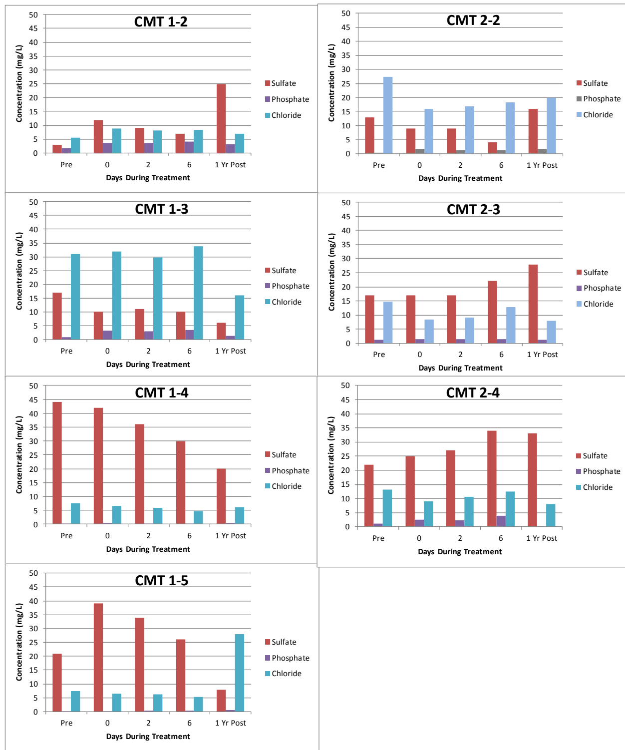
Figure 5-45. Concentrations (mg/L) of common anions measured in CMT 1 and CMT 2 at each depth.
