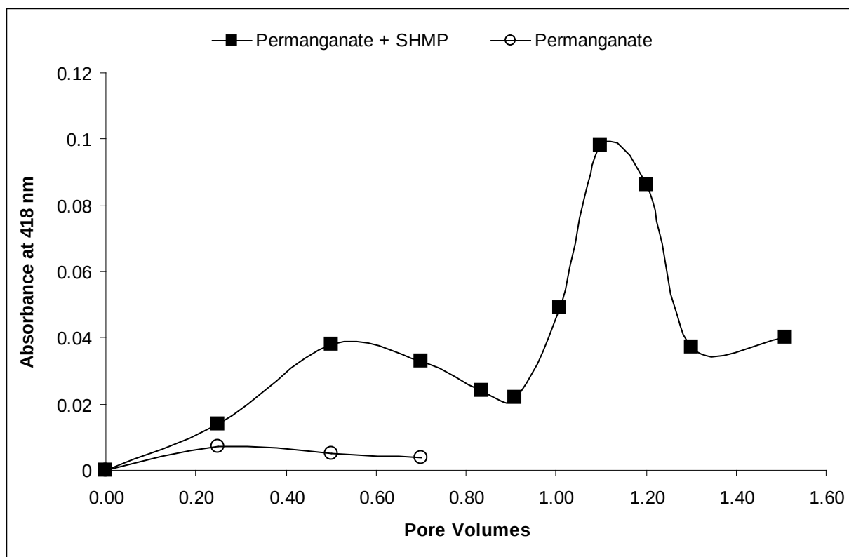
Figure 28. Column effluent absorbance at 418 nm – indicator of dissolved or suspended \text{MnO}_2 concentration passing through column
