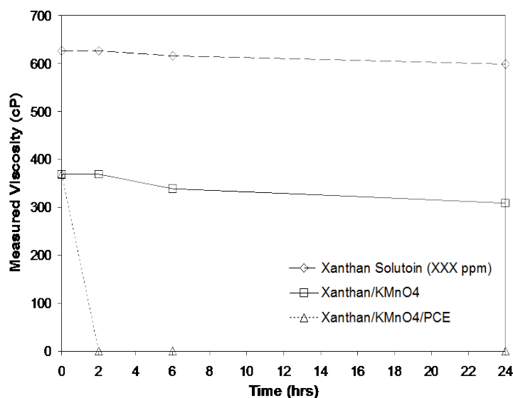
Figure 2-2. Viscosity-time plot.
