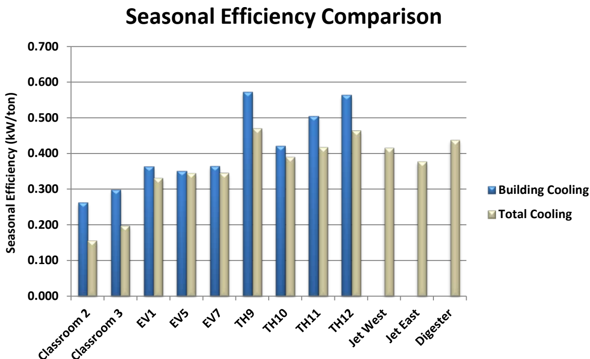
Figure 7. Coolerado seasonal efficiency comparison.
