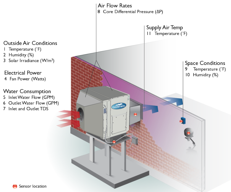
Figure 6. Coolerado DAS. (Source: Joshua Bauer, NREL)
