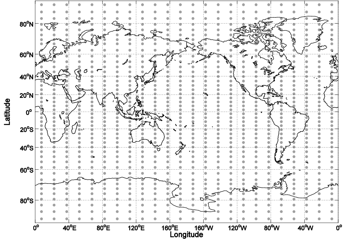
Figure 5. Global grid spacing of the GAIM-GM model. Each gray dot represents the coordinates of model output data. Spatial resolution is 4.667° latitude (3° latitude poleward of 70°) by 15° longitude.
