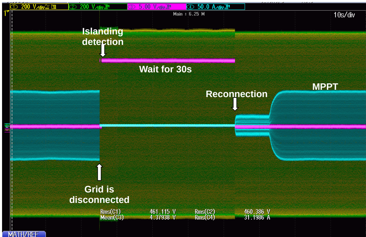
Figure 6. Grid disconnection and reconnection tested at McGuire AFB.
