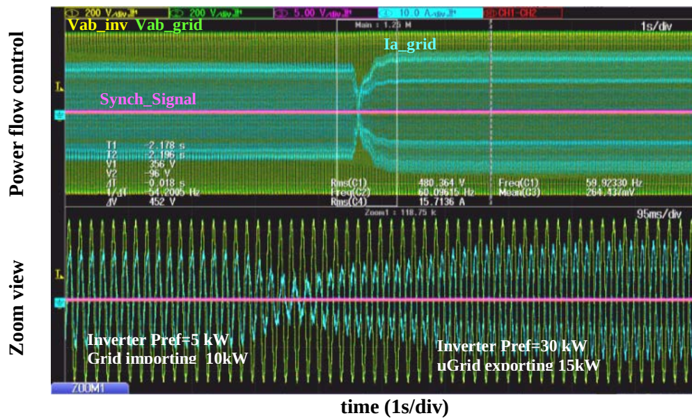
Figure 5. Power flow control.
