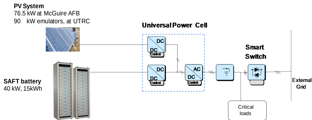
Figure 2. Schematic diagram of the energy microgrid system and sub-system installed at McGuire AFB.
