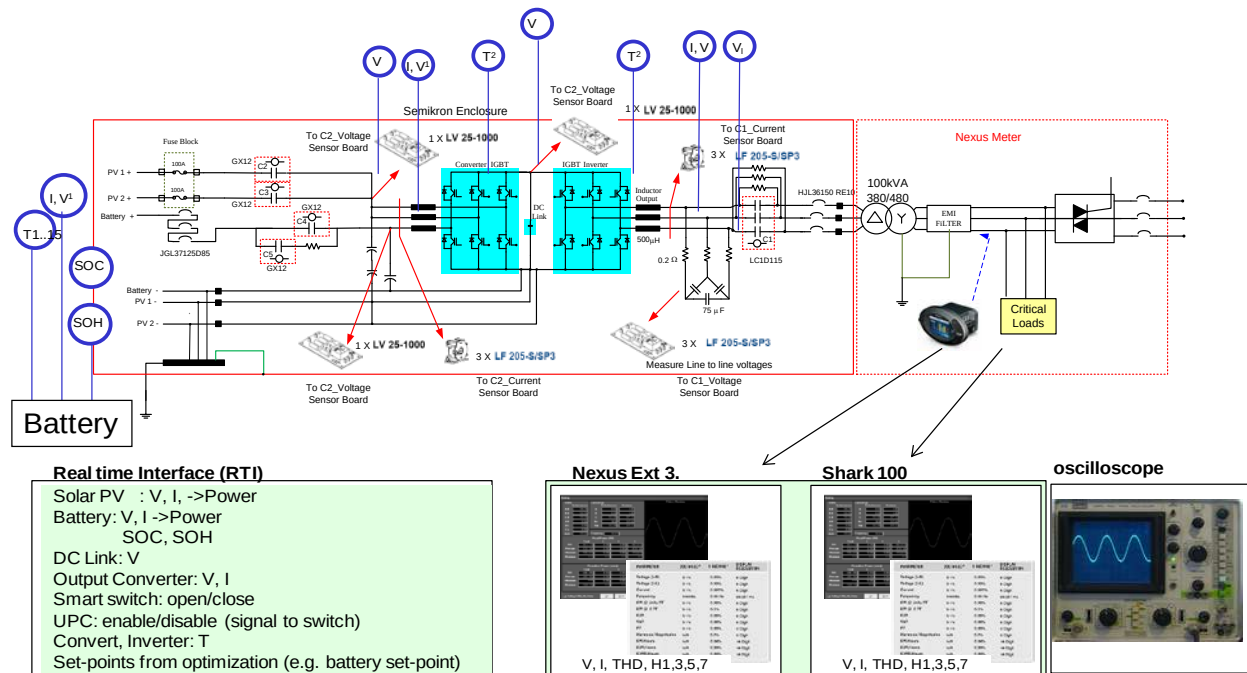
Figure 3. Microgrid demo sensors – type and location.
