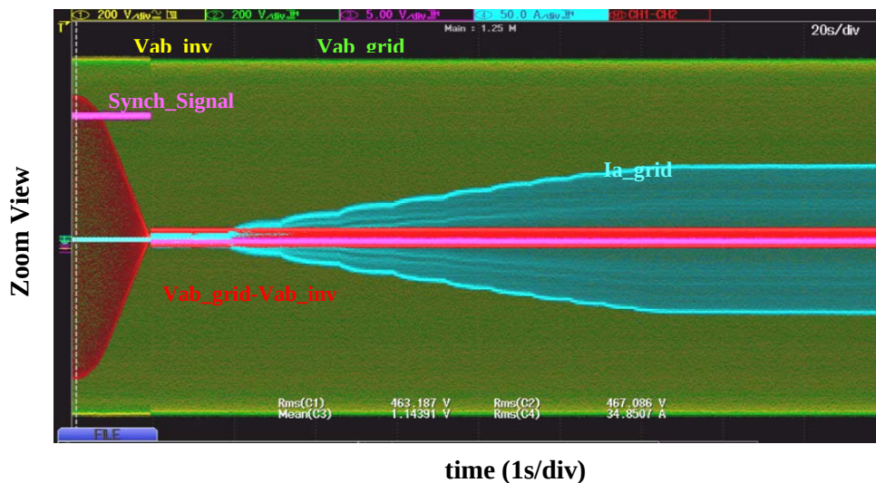
Figure 4. Grid synchronization at McGuire AFB.
