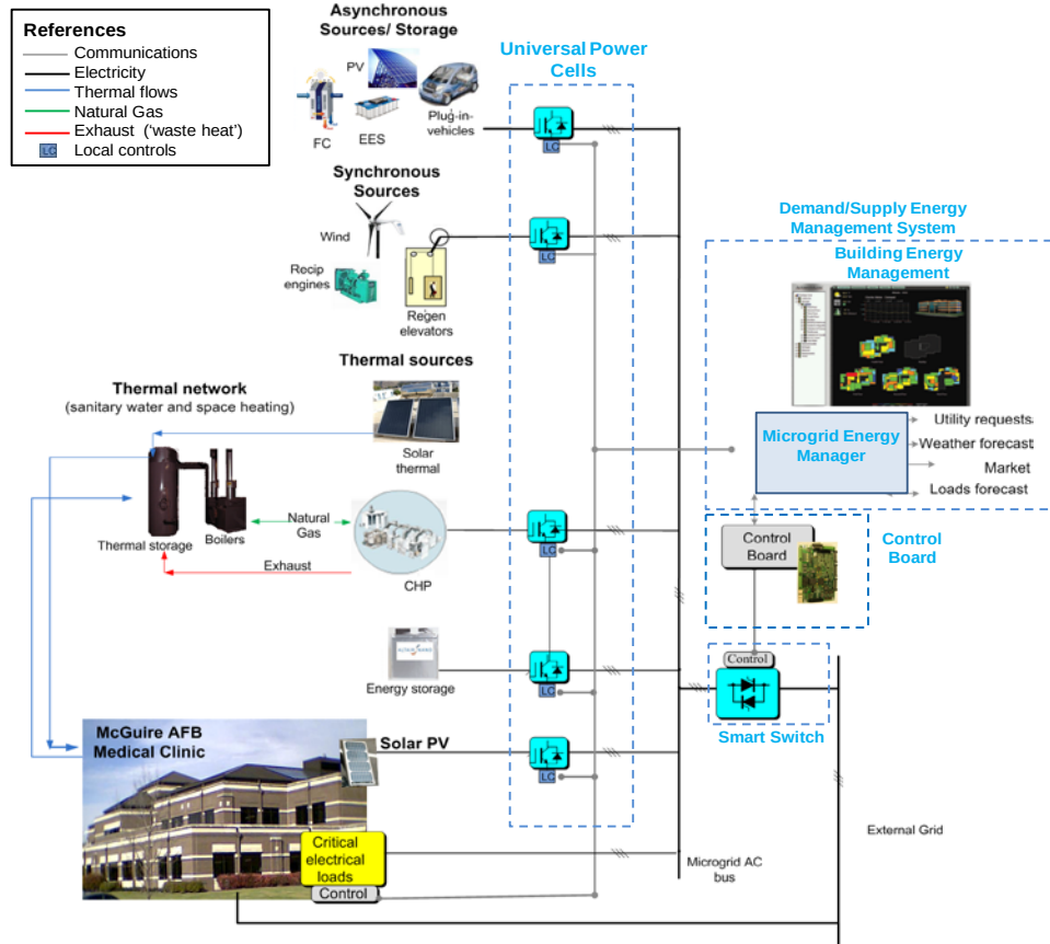
Figure 1. UTRC energy microgrids concept.
