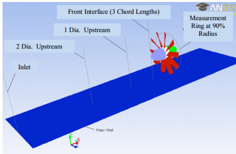
Figure 16: The configuration of the rotor and wall in which both potential and shear flows were modeled.
