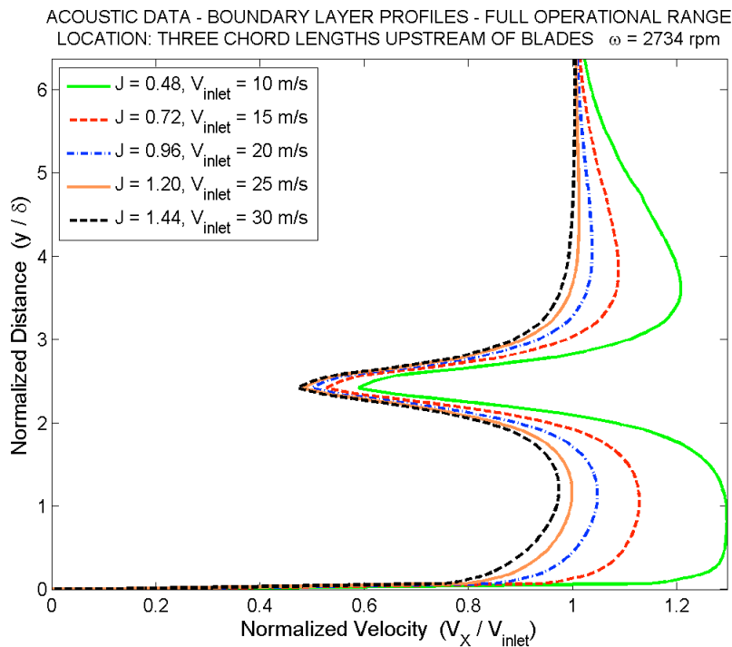
Figure 2.18 – Acoustic: BL Profile at 3 Chord Lengths Upstream for All Case Files
