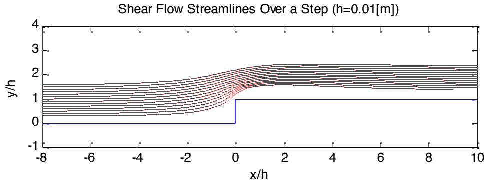
Figure 14: Shear flow streamlines over a forward-facing step. The shear flow is modeled by solutions to the RANS equations.
