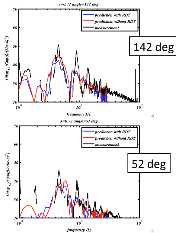
Figure 4.5: Predicted and measured spectra at J=0.72 for a thrusting rotor at 142^\circ and 52^\circ to the rotor axis. Predictions with and without RDT are shown.
