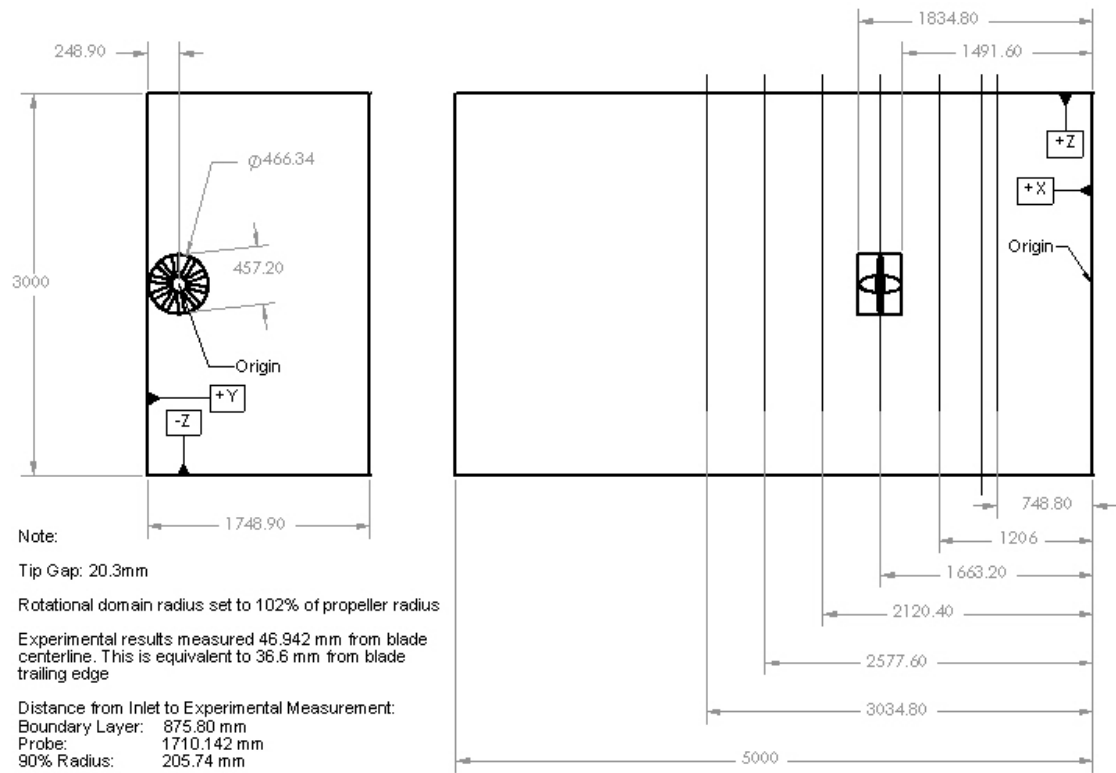
PROPELLER AND TUNNEL - CONFIGURATION 3
