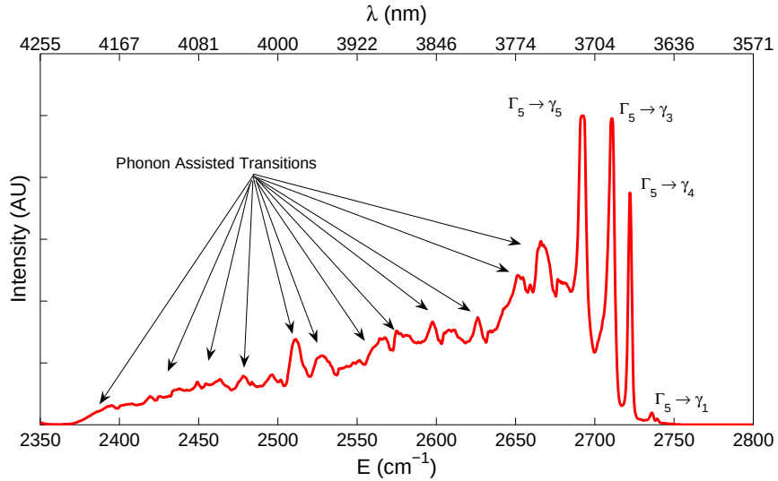
Figure 19. The laser-induced fluorescence spectrum of Fe:ZnSe at 5 K.
