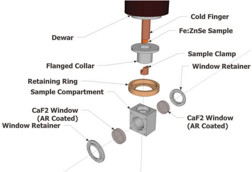
Figure 40. A breakout view of the revised sample compartment.
