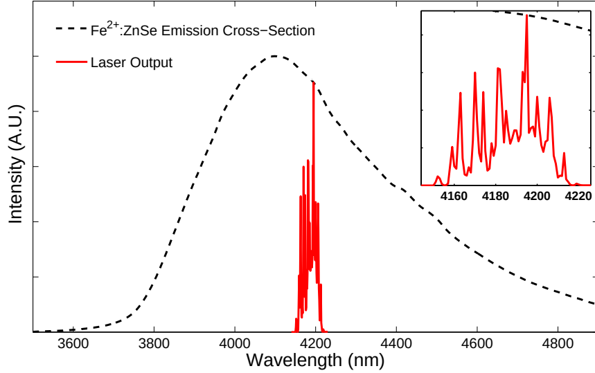
Figure 36. The normalized emission spectrum of the Fe:ZnSe laser operating at full power. The black dotted line is the normalized emission cross-section at \sim 80\ \text{K} as calculated from a system-compensated emission spectrum and the F  chtbauer–Ladenburg equation. The structure in the output is hypothesized to be due to mode-hopping. The inset shows the lasing region in greater detail.
