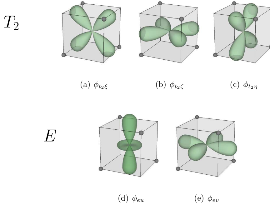
Figure 3. Wavefunctions for the L = 2 states of the d^6 configuration in a tetrahedrally coordinated environment. The origin of the state labels is discussed in Subsection 2.3.5.
