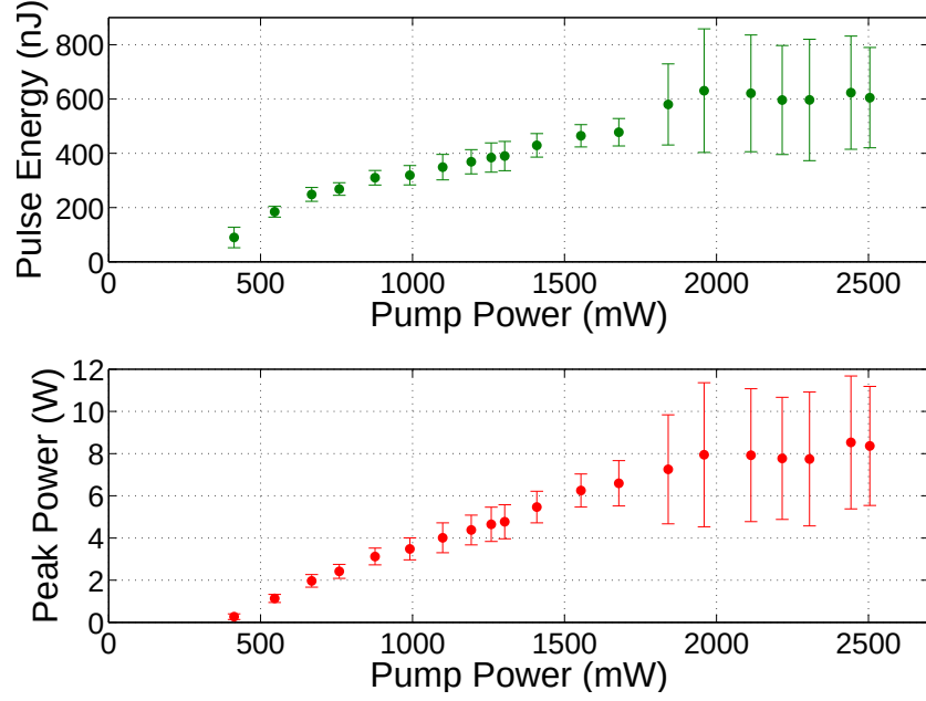
Figure 48. The average pulse energy and peak power of the laser with respect to pump power.
