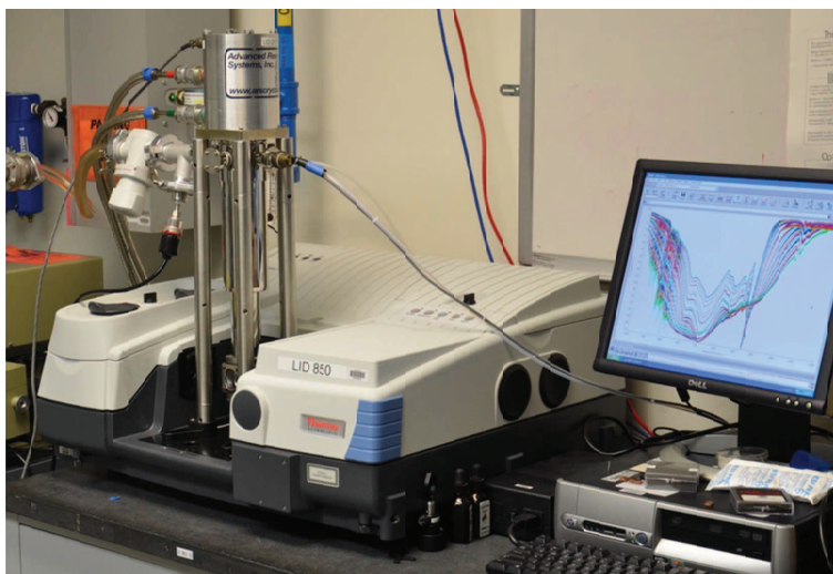
Figure 12. The ARS cryostat in the sample compartment of a Nicolet 6700 FTIR.
