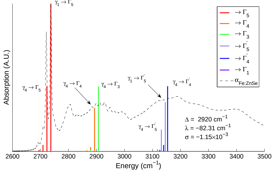
Figure 14. The fit of the eigenvalues of the electronic states of \text{Fe}^{2+} ions to the absorption spectrum of \text{Fe:ZnSe} at T = 10 K.
