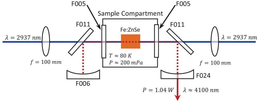
Figure 41. A U-cavity design for a CW Fe:ZnSe laser. Note that the smaller sample compartment permits the addition of turning mirrors.
