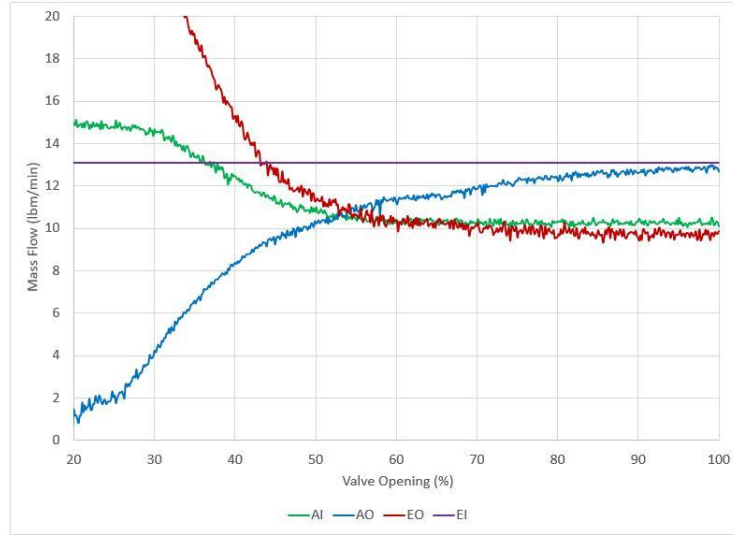
Figure 24: Comprex data point at elevated temperatures with best mass flow matching
