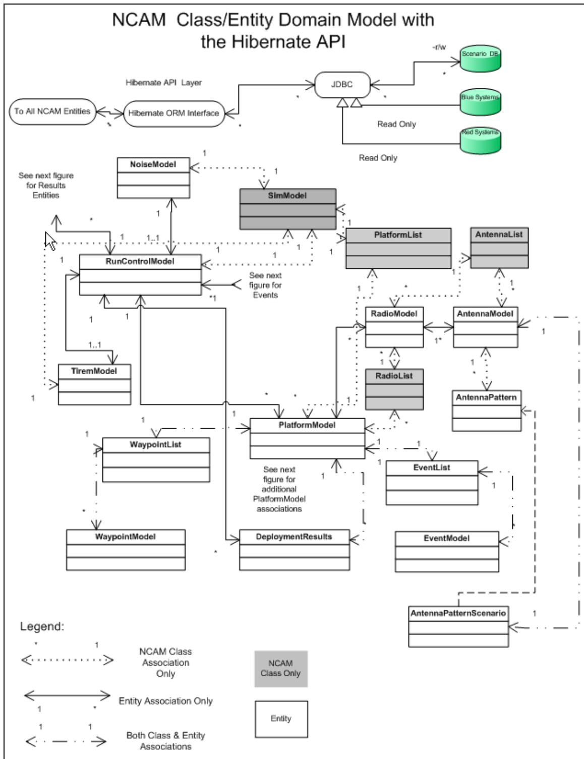
Figure 2. NCAM class/entity model.
