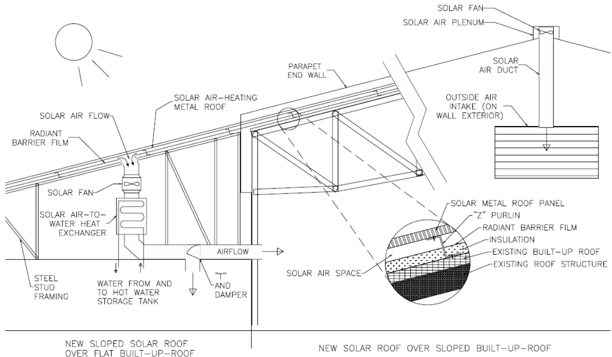
Figure A-1 , 1 Concept Schematic Section
