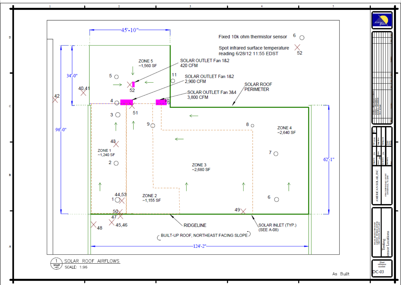
Figure A-1, 15 Sensor Location Plan
