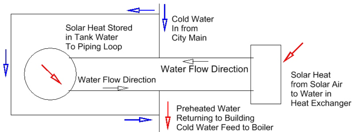
Figure A-1, 4 Parallel Piping Schematic
