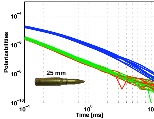
(e) 25 mm projectile.
