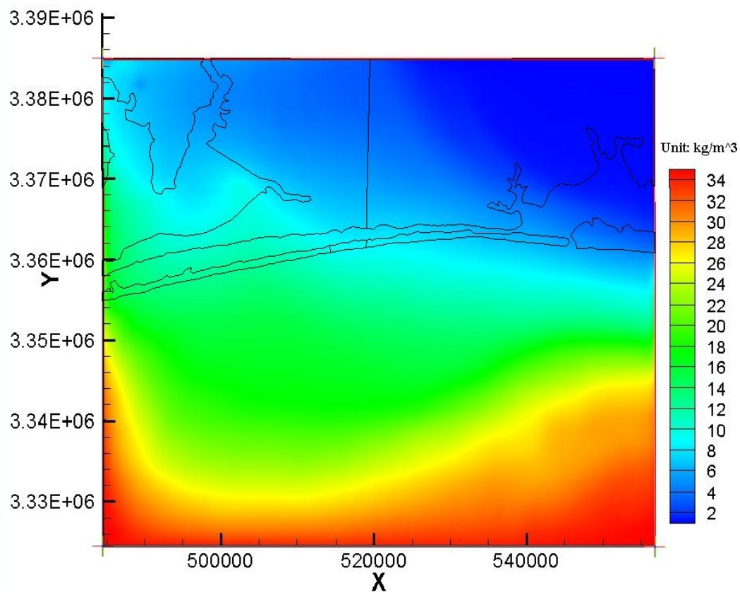
Figure 4.5.8. Pre-development salinity distribution in the lower Floridan Aquifer.
