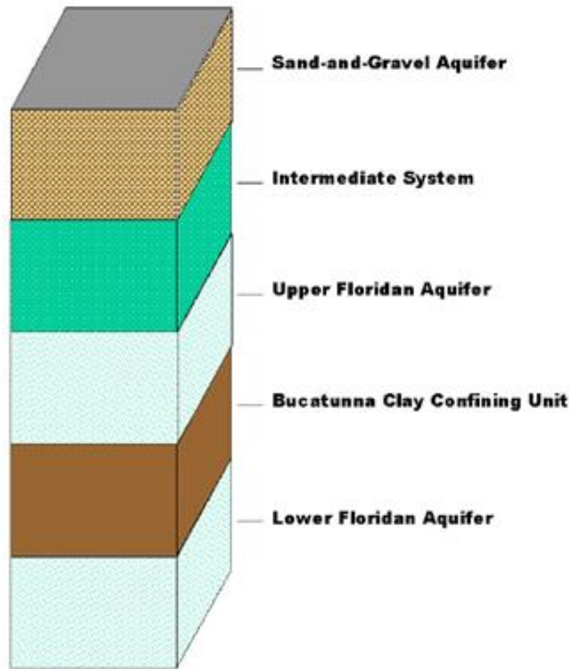
Figure 3.5.4. Hydrogeologic units in the study area (NFWWMD, 2000).
