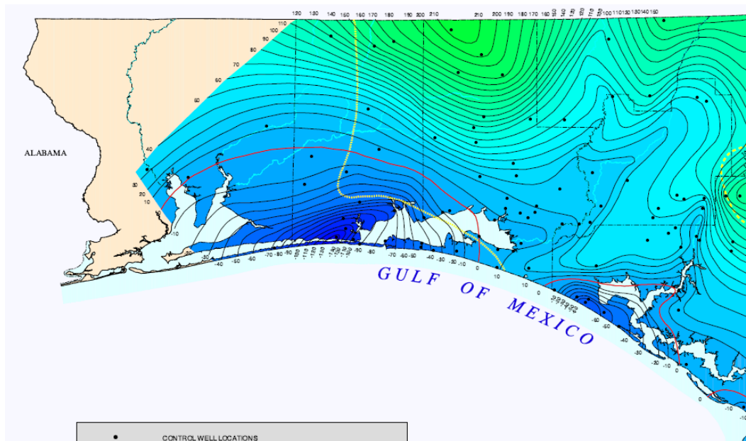
Figure 4.5.10. Potentiometric surface of the Floridan Aquifer system, 1998 (contours in feet) (Maloney et al., 1998).
