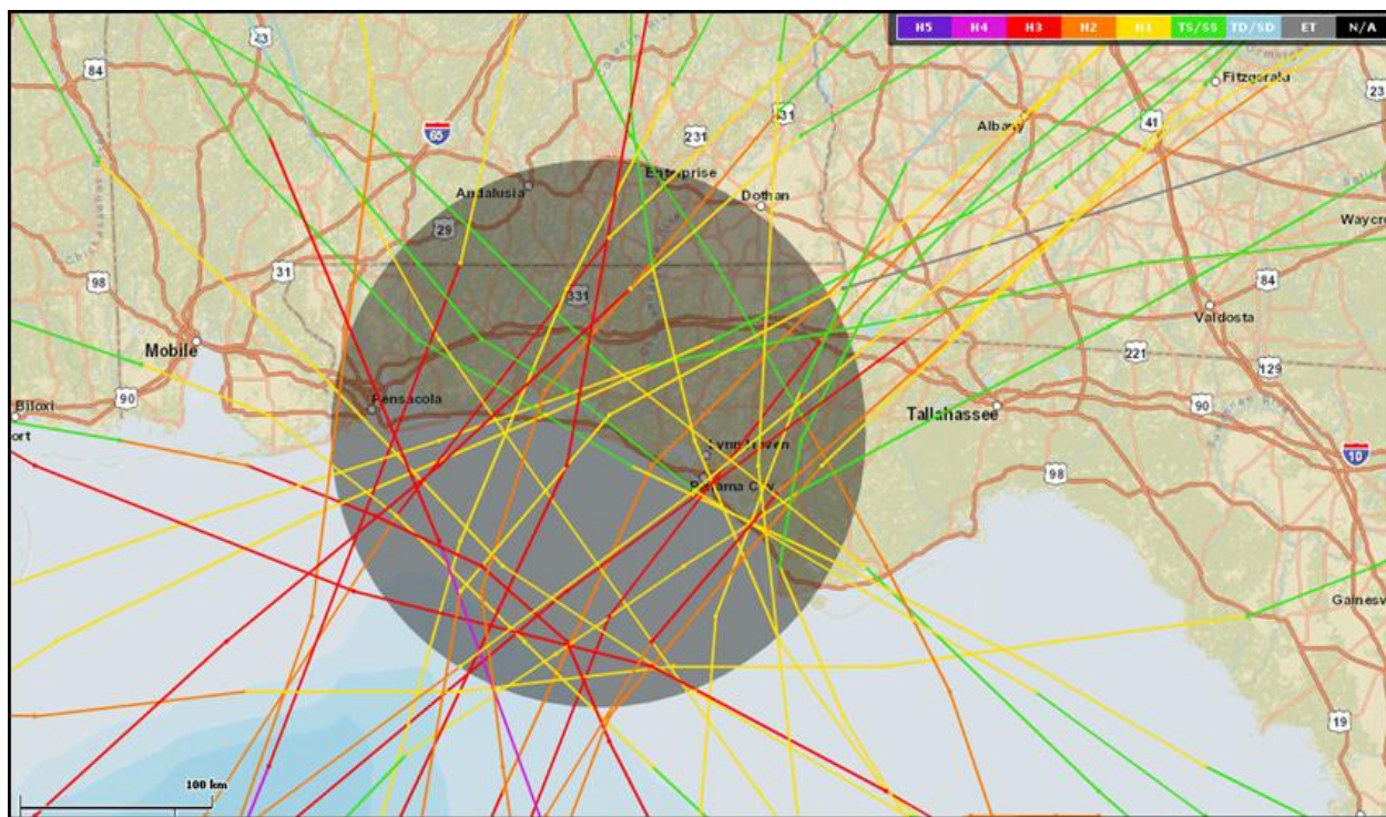
Figure 3.3.1. Tracks of the 32 hurricanes (Cat. 1-5) which have passed within a 140-km radius of the study area at the eastern margin of Eglin AFB (Lat. 30.3265 N, Lon. 86.1510 W), 1851-present. (Source: NOAA, 2012a).
