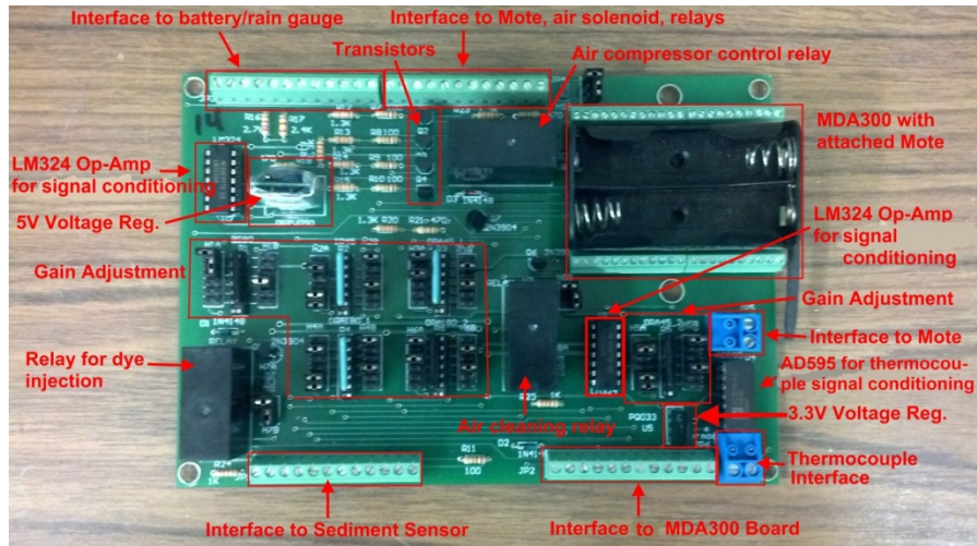
Figure 2.10 PCB control board
