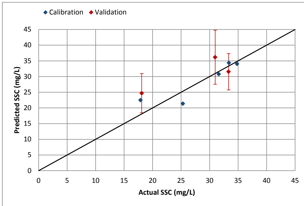
Figure 6.35 Predicted SSC vs. actual SSC of the calibration and validation data sets for the Upatoi North sensor site using OR180 linear calibration model
