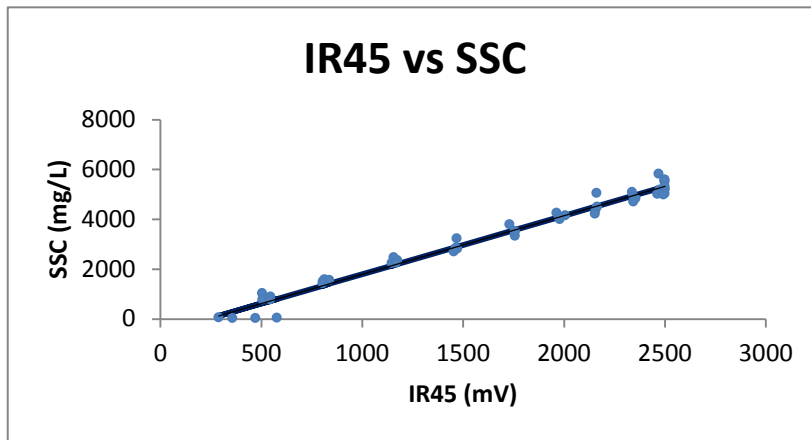
Figure 2. SSC linear model of the sensor in Little Kitten using IR45 signal
