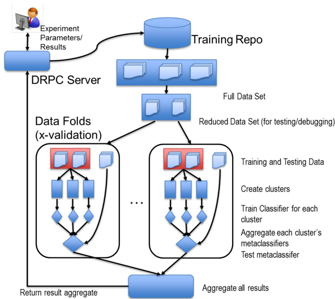
Figure 4. Scalable Training
