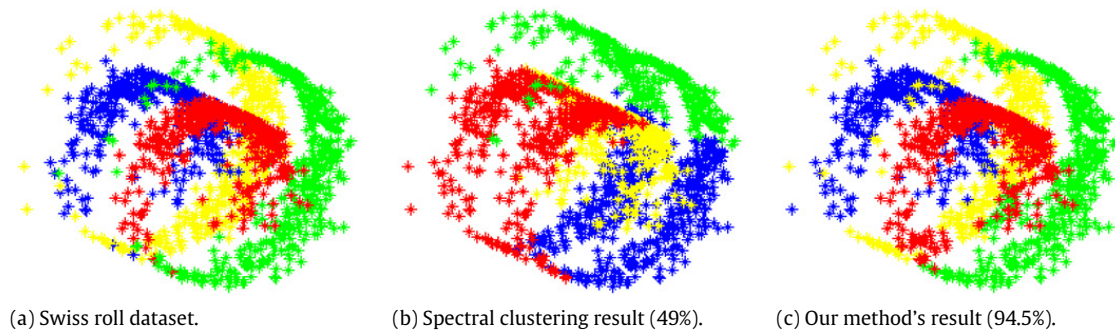
Fig. 1. Swiss roll dataset results.
