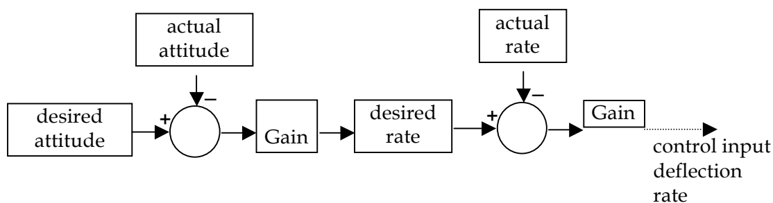
Figure 18. Attitude control via proportional controllers in series
