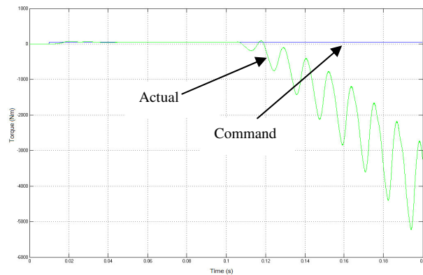
(a) Torque signal.
