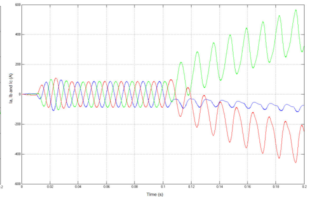
(b) Ia, Ib and Ic signals
