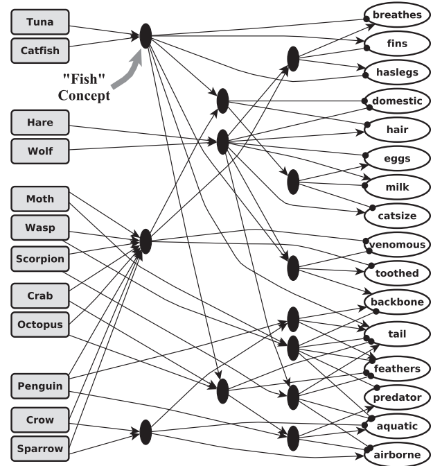
Fig. 2 Part of the zoo ontology. Instances are individual animals shown on the left, and base-level features are on the right. Black nodes in the middle correspond to higher-level features. The concept that corresponds to "fish" is marked. Inhibitory links (for negative features, such as \neg \text{fins} ) are shown as dark circles.
