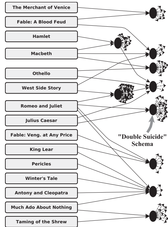
Fig. 8 Part of the ontology Spontol learned from the story dataset. As in the zoo ontology in Fig. 2, black ovals represent higher level concepts. The “raw” features (corresponding to the white ovals in Fig. 2) are omitted due to space limitations. Instead, we show the outgoing edges from each black oval. While in the zoo ontology, the higher level concepts correspond to shared surface features, in this figure, high level concepts correspond to shared structural features, or analogical schemas . For example, the denoted oval on the right represents a Double Suicide schema, which happens in both Romeo and Juliet and in Julius Caesar .
