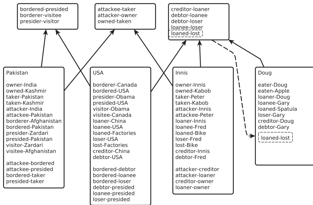
Fig. 9 Basic inference using bottom-up parsing, top-down prediction, and chaining. In this simplified example, we use an ontology of schemas (learned from stories shown on the lower left) to parse The Story of Doug, which is parsed to inherit from the concept at the top-right. This concept has the atomic feature “loaned-lost”, which, through top-down implication, we infer to be part of The Story of Doug. We then use our chaining system to interpret the features in the Story of Doug as bindings, and chain “loaned-lost” with “loaned-Spatula” to infer “lost-Spatula” (i.e., the Spatula was lost).
