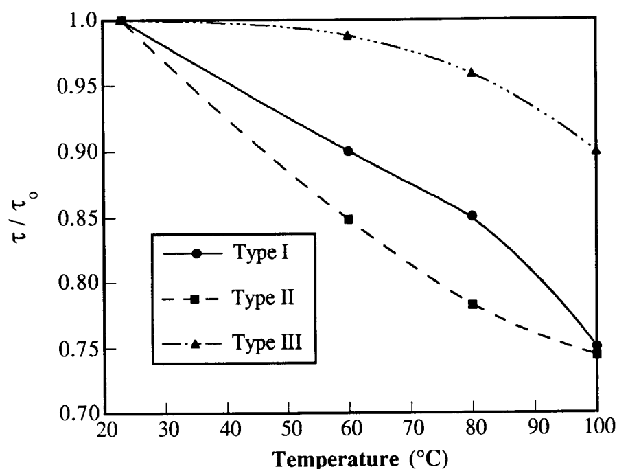
Fig. 3 Variation of normalized interfacial shear strength ( \tau/\tau_0 ) with temperature for the three types of samples.
