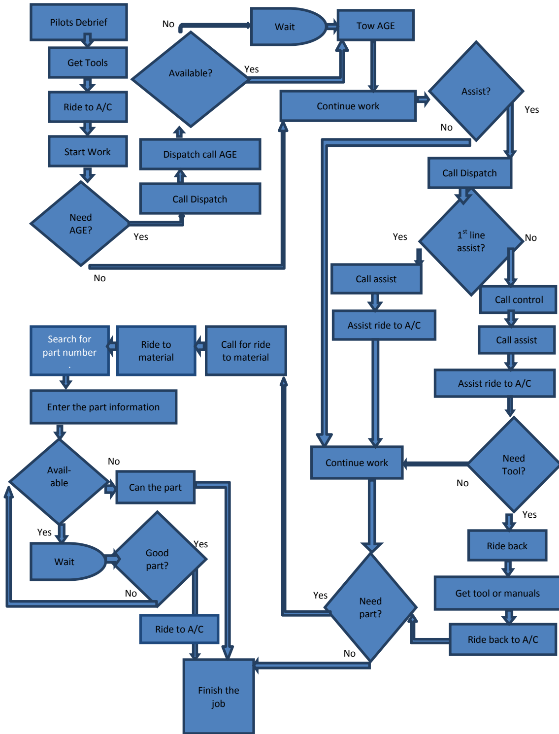
Figure 17. F-15 Maintenance Process Flow
