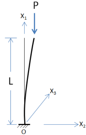
Figure 12: Fixed Column Subjected to a Concentrated Load
