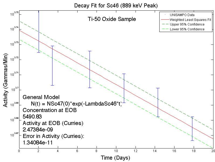
Figure 61. This figure, generated in MATLAB from the peak fitting data extracted by the UNISAMPO data analysis tool shows a weighted nonlinear model fit of the 889 keV peak of 46 Sc within the 50 Ti sample. It is plotted with 95% confidence bounds determined by error propagated throughout the fitting process.
