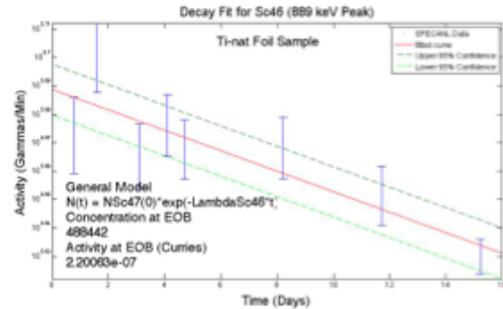
Figure 38. A comparison of analysis tool results for 889 keV 46 Sc Peak in nat Ti shows that there is no specific trend for the data leading to the conclusion that the variances in the data are a product of poor statistics.
