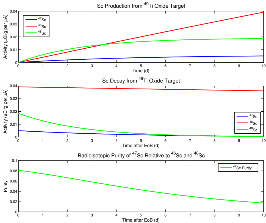
Figure 11. These plots were generated in the MATLAB script found in Appendix D. The calculations are based on production rates for a ^{49}\text{Ti} target produced in Cinder90. The graph on the top shows the relative production of isotopes over the course of a 10-day irradiation. The middle graph shows relative decay rates as a function of time after the end of irradiation. The graph on the bottom shows the relative isotopic purity of ^{47}\text{Sc} .
