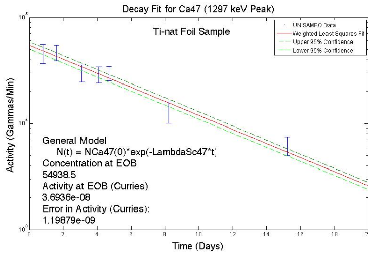
Figure 47. This figure, generated in MATLAB from the peak fitting data extracted by the UNISAMPO data analysis tool shows a weighted nonlinear model fit of the 1297 keV peak of ^{47}\text{Ca} within the ^{nat}\text{Ti} sample. It is plotted with 95% confidence bounds determined by error propagated throughout the fitting process.
