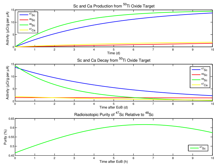
Figure 44. These plots were generated in the MATLAB script found in Appendix D. The calculations are based on production rates determined from experimental results. The graph on the top shows the relative production of isotopes over the course of a 10-day irradiation. The middle graph shows relative decay rates as a function of time after the end of irradiation. The graph on the bottom shows the relative isotopic purity of ^{47}\text{Sc} .
