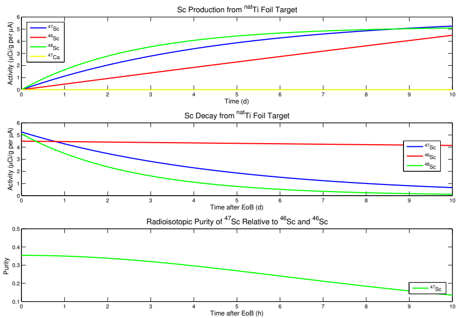
Figure 16. These plots were generated in the MATLAB script found in Appendix D. The calculations are based on production rates for a ^{nat}\text{Ti} target produced in MCNP6. The graph on the top shows the relative production of isotopes over the course of a 10-day irradiation. The middle graph shows relative decay rates as a function of time after the end of irradiation. The graph on the bottom shows the relative isotopic purity of ^{47}\text{Sc} .
