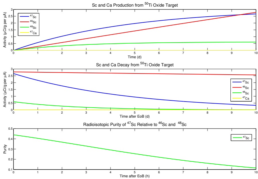
Figure 18. These plots were generated in the MATLAB script found in Appendix D. The calculations are based on production rates for a ^{50}\text{Ti} target produced in MCNP6. The graph on the top shows the relative production of isotopes over the course of a 10-day irradiation. The middle graph shows relative decay rates as a function of time after the end of irradiation. The graph on the bottom shows the relative isotopic purity of ^{47}\text{Sc} .
