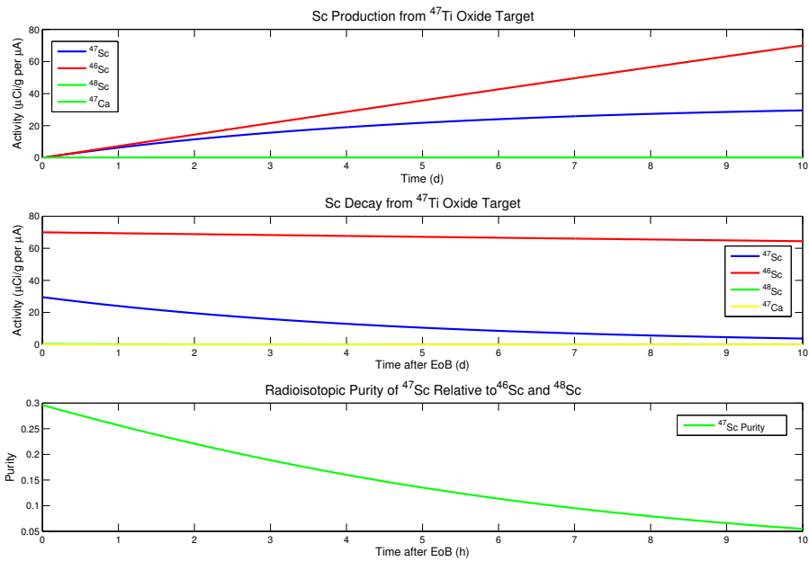
Figure 17. These plots were generated in the MATLAB script found in Appendix D. The calculations are based on production rates for a ^{47}\text{Ti} target produced in MCNP6. The graph on the top shows the relative production of isotopes over the course of a 10-day irradiation. The middle graph shows relative decay rates as a function of time after the end of irradiation. The graph on the bottom shows the relative isotopic purity of ^{47}\text{Sc} .
