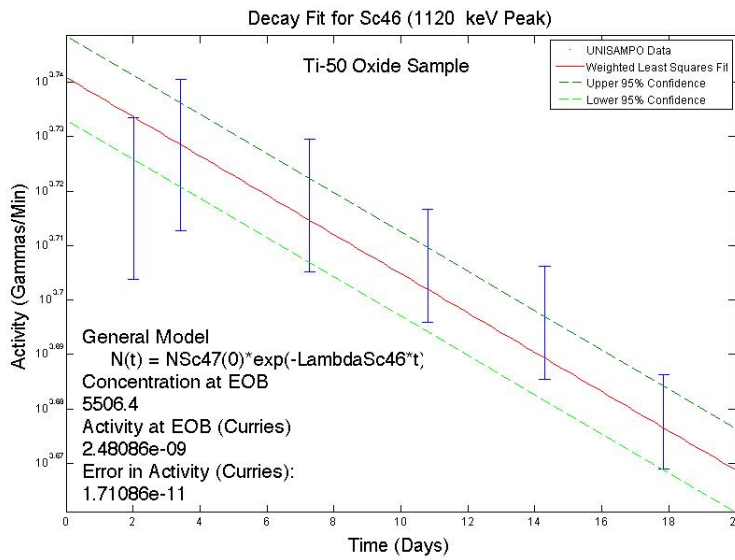
Figure 57. This figure, generated in MATLAB from the peak fitting data extracted by the UNISAMPO data analysis tool shows a weighted nonlinear model fit of the 1120 keV peak of ^{46}\text{Sc} within the ^{50}\text{Ti} sample. It is plotted with 95% confidence bounds determined by error propagated throughout the fitting process.
