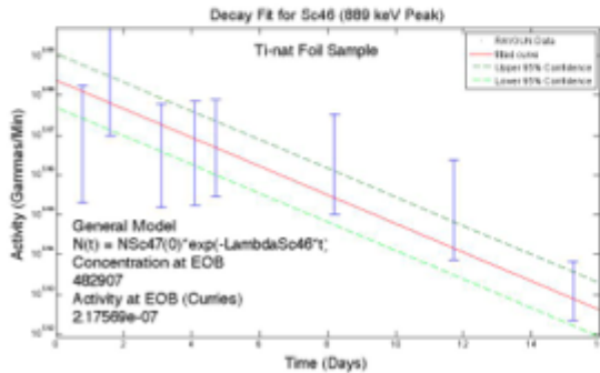
Figure 38. A comparison of analysis tool results for 889 keV 46 Sc Peak in nat Ti shows that there is no specific trend for the data leading to the conclusion that the variances in the data are a product of poor statistics.
