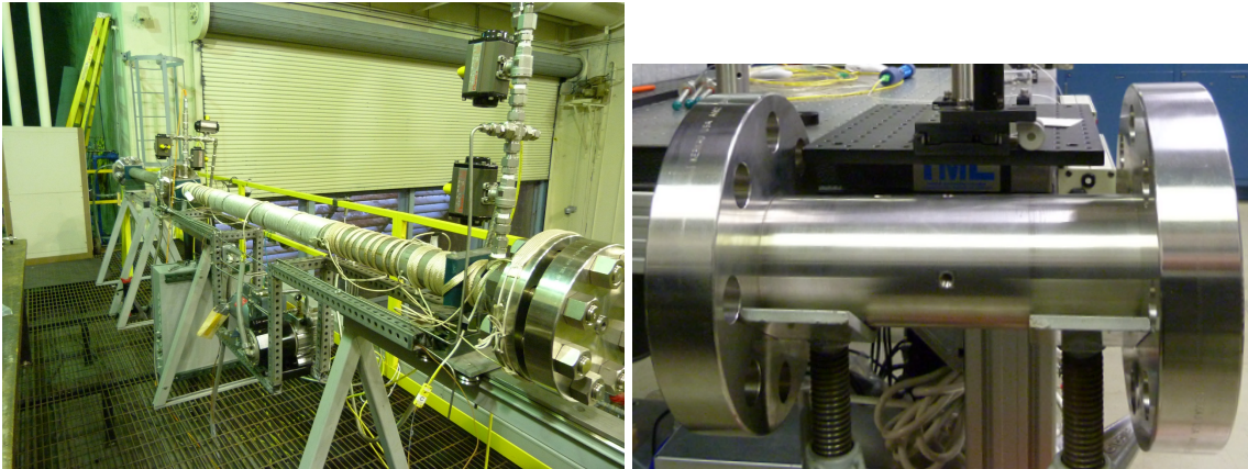
(a) Detonation tube.
