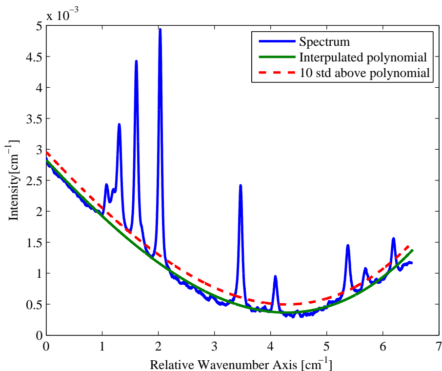
Figure 4.8: This figure depicts a third order polynomial fit to the minimums of a spectrum. The red dotted line shows the region which is ten standard deviations of the noise above the polynomial.
