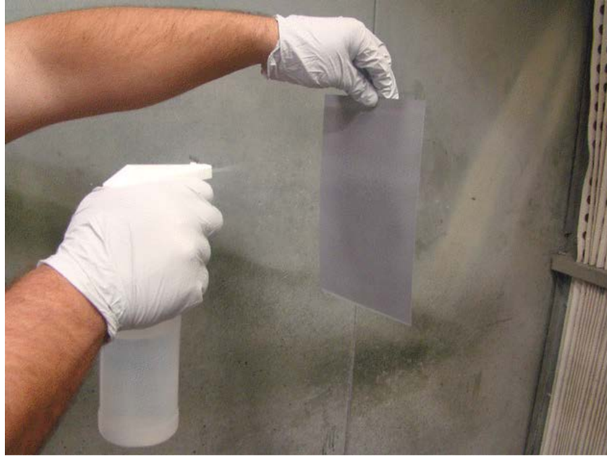
Figure 6. Image of the spray application of GPS silane to the 2024-T3 aluminum alloy flexible adherend.
