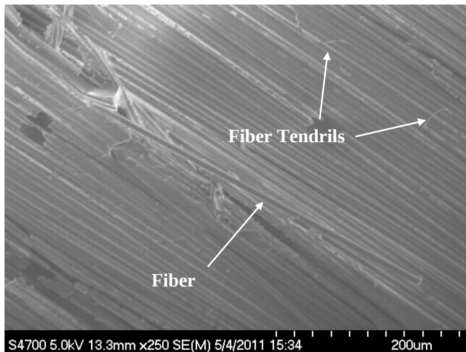
Figure 15. SEM image of composite surface prepared with Bleeder Lease C at 250× magnification.
