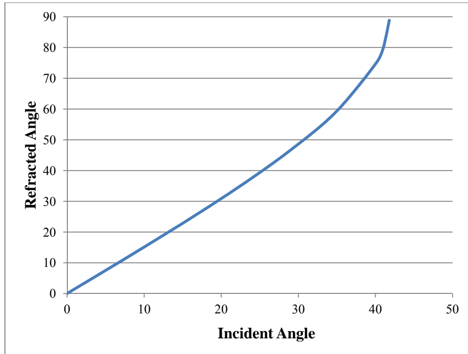
Figure 6. Refraction angle dependence on angle of incidence due to internal reflection of a material with n=1.5 from which light propagates into a gas with n=1 . Refraction angle greater than 90 degrees denotes the light is internally reflected inside material 1 versus passing into material 2.
