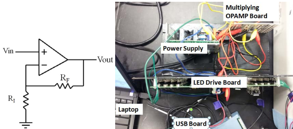
Figure 19. Input voltage multiplying OPAMP schematic and diagram
