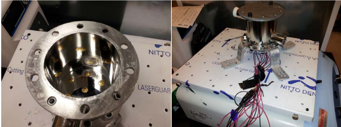
Figure 18. Reactor vessel with flow through pipe sealed
